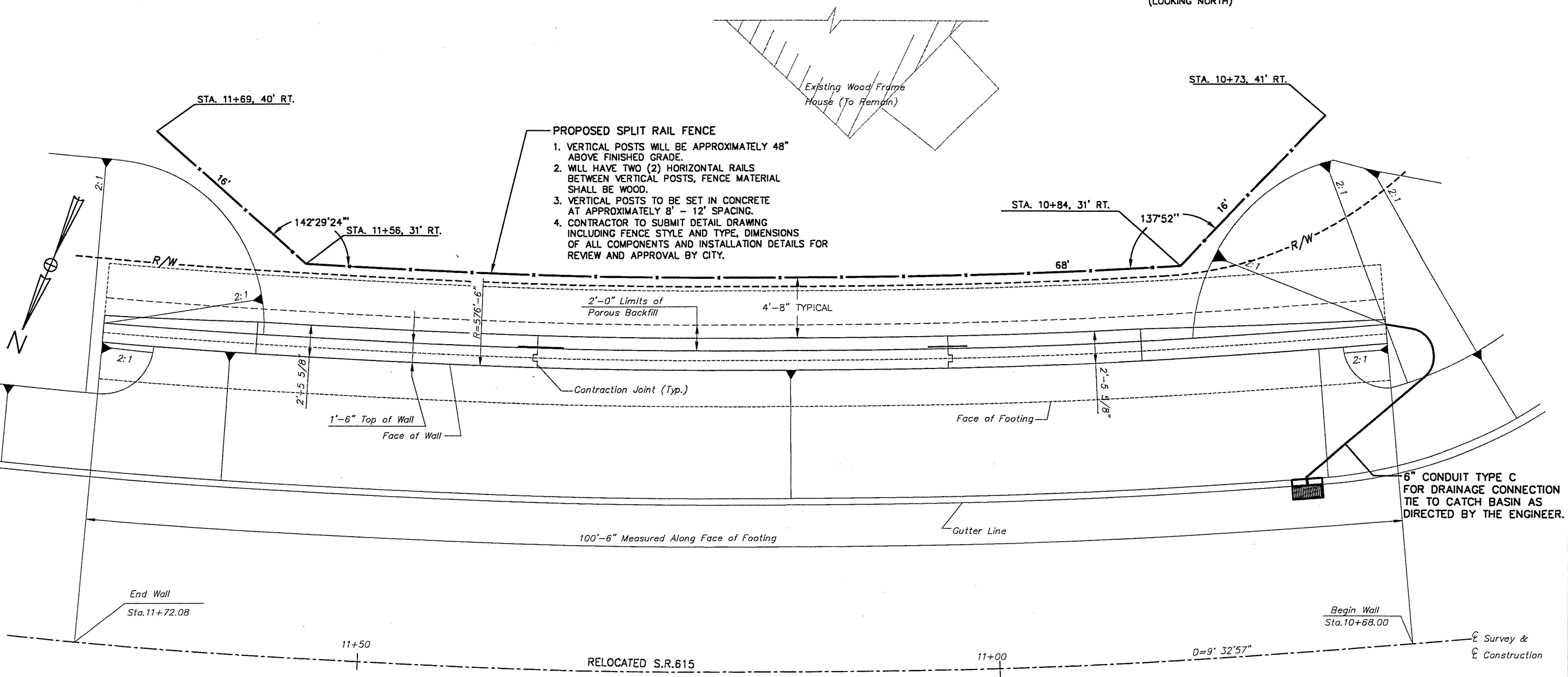
RETAINING WALL PLAN
