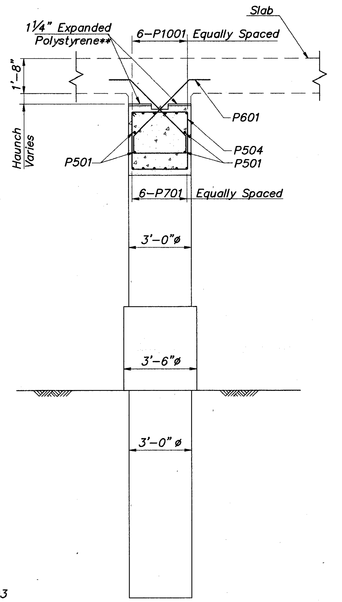
SECTION J-J
