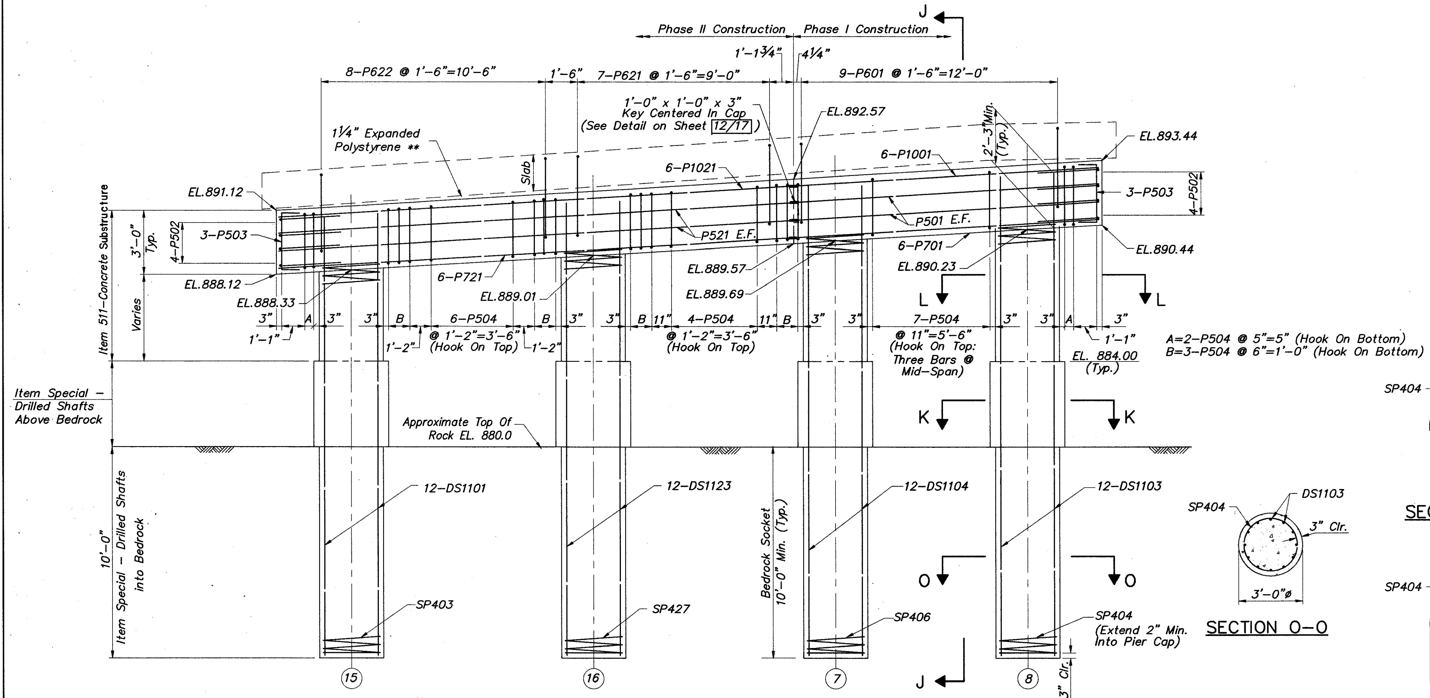
PIER 2 ELEVATION
