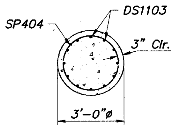
SECTION O-O
