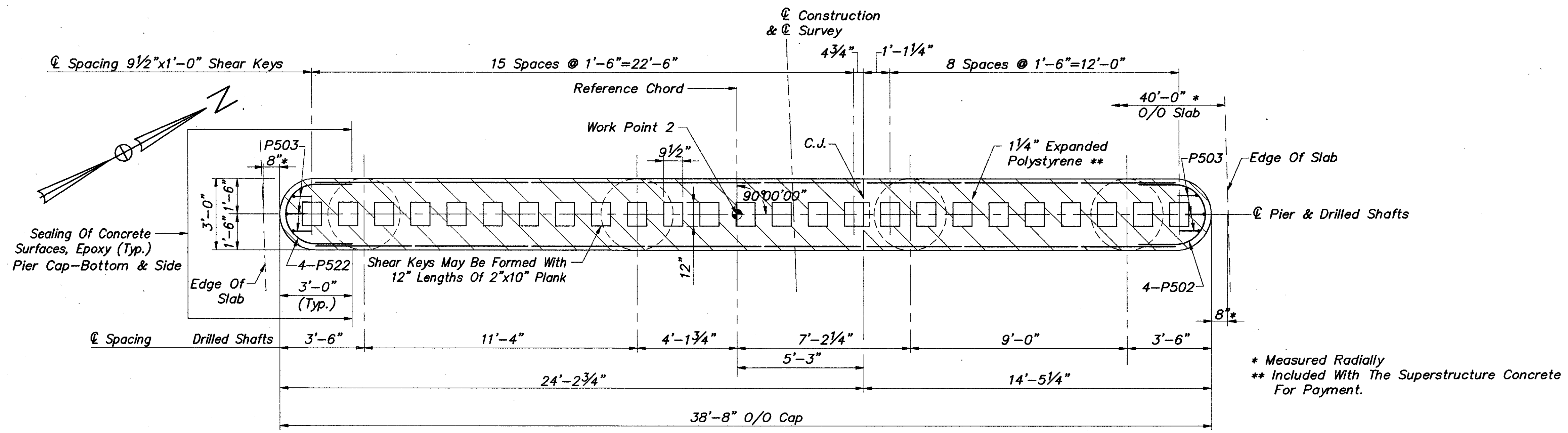
PIER 2 PLAN
