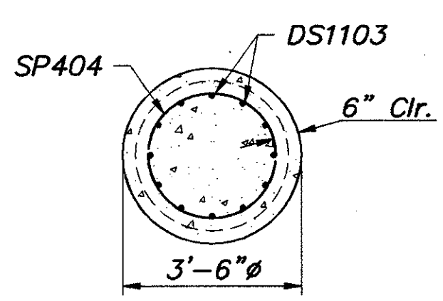
SECTION K-K
