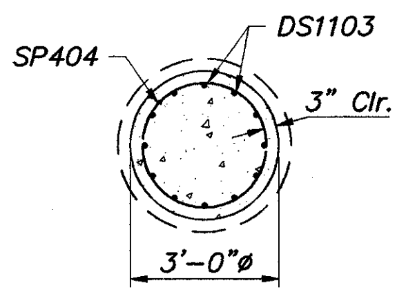
SECTION L-L
