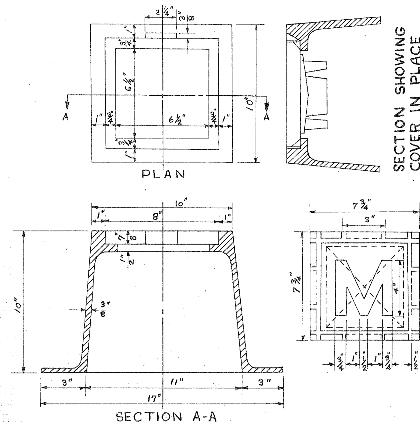
MONUMENT FRAME & COVER C.I. Scale 3" = 1'-0"
