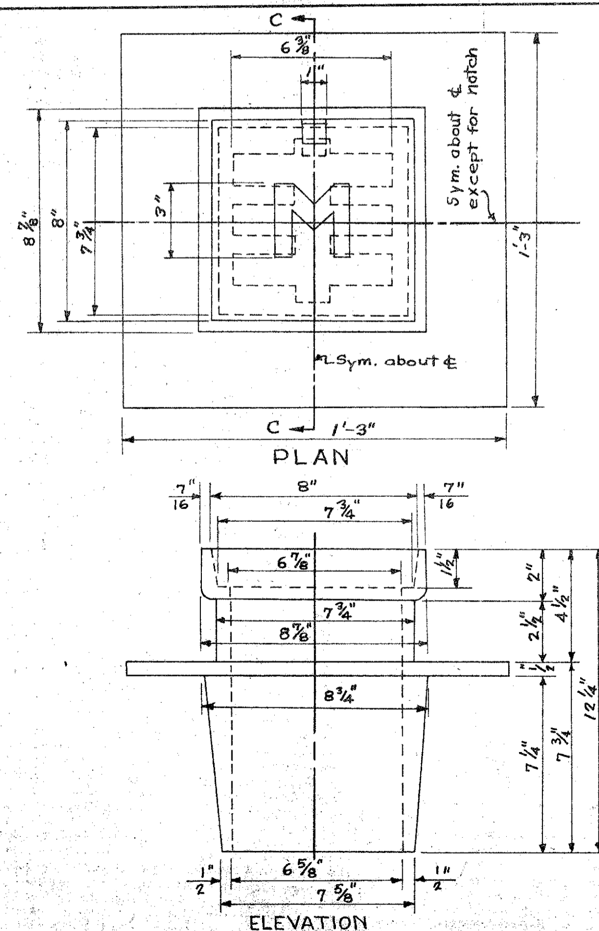
MONUMENT FRAME & COVER C.I. Scale 3" = 1'-0"
