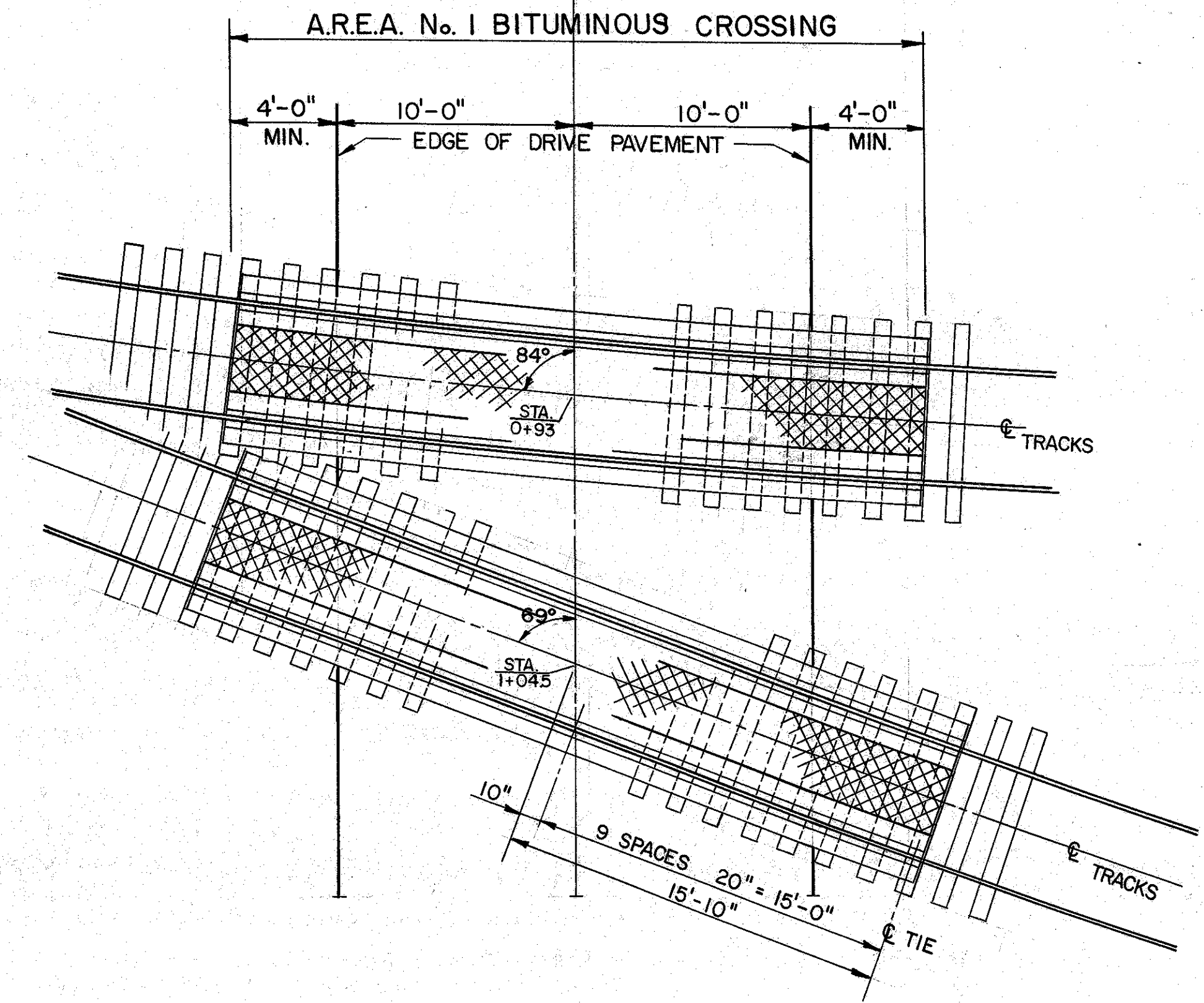
U.S.I. SIDING / CHEMICAL COMPANY DRIVEWAY SCALE: 1" = 5'-0" (WATER STREET STATION: 116+10)
