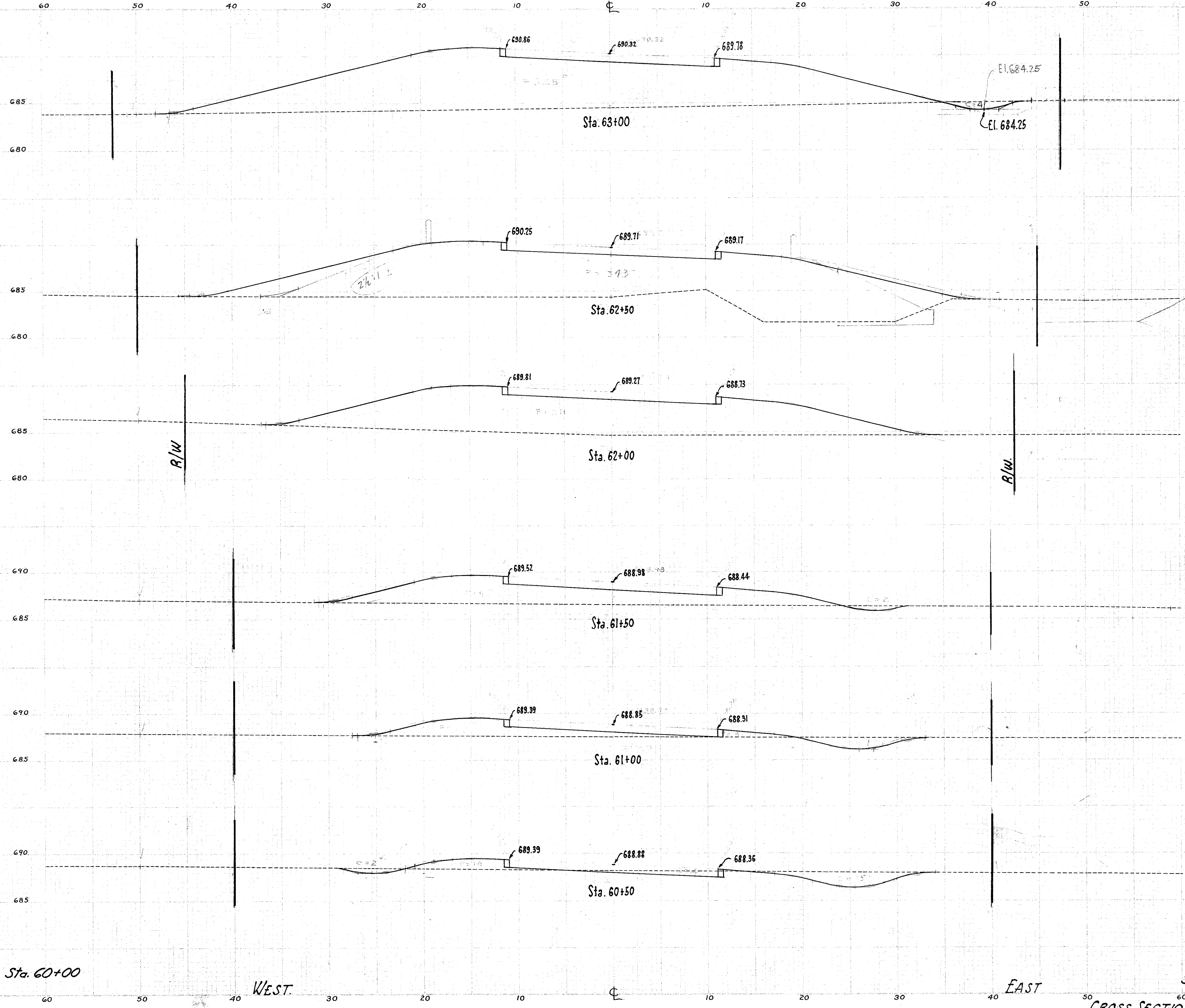
CROSS SECTIONS FROM STA. 60+50 TO STA. 63+00
