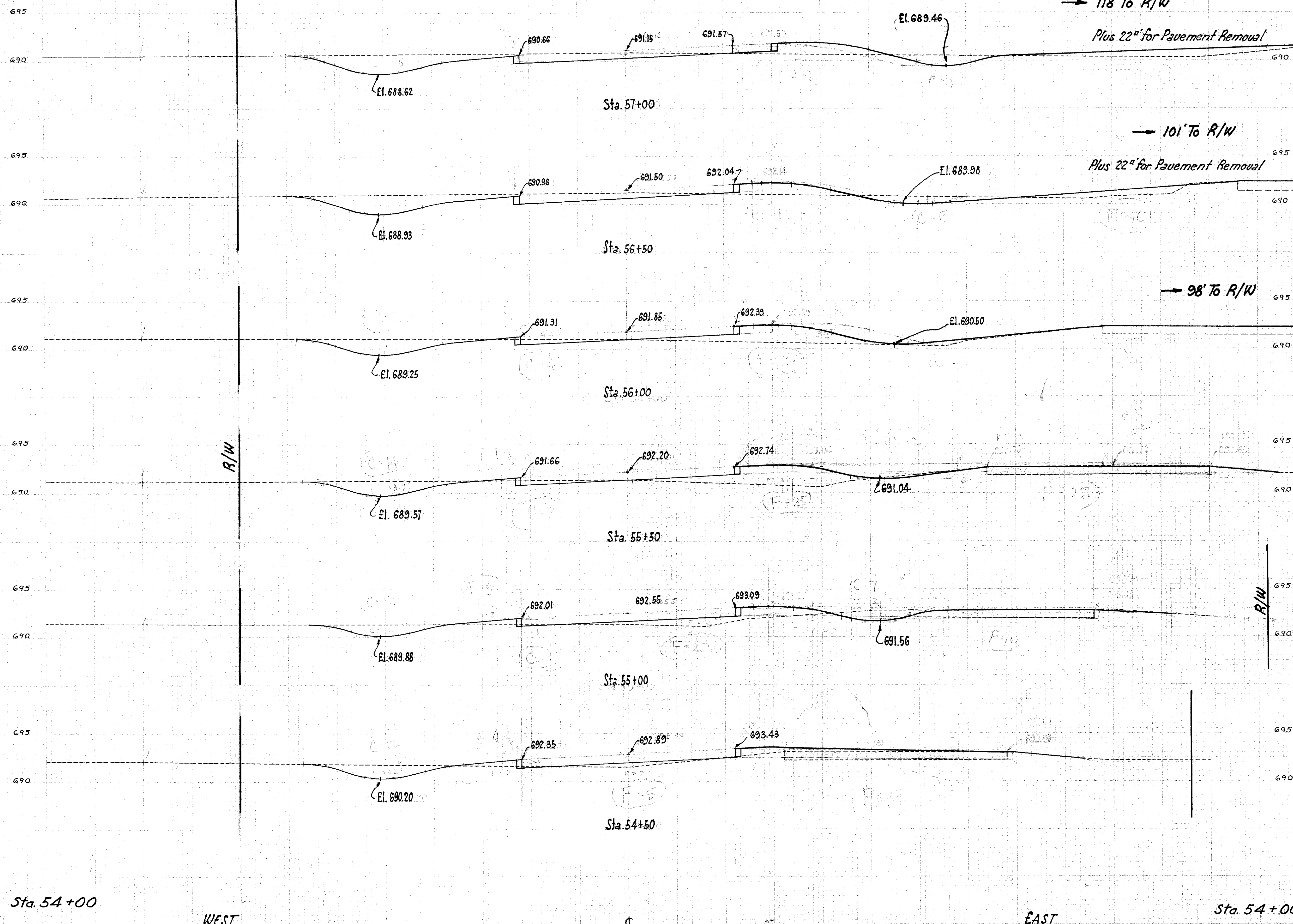
CROSS SECTIONS FROM STA. 54+50 TO STA. 57+00.
