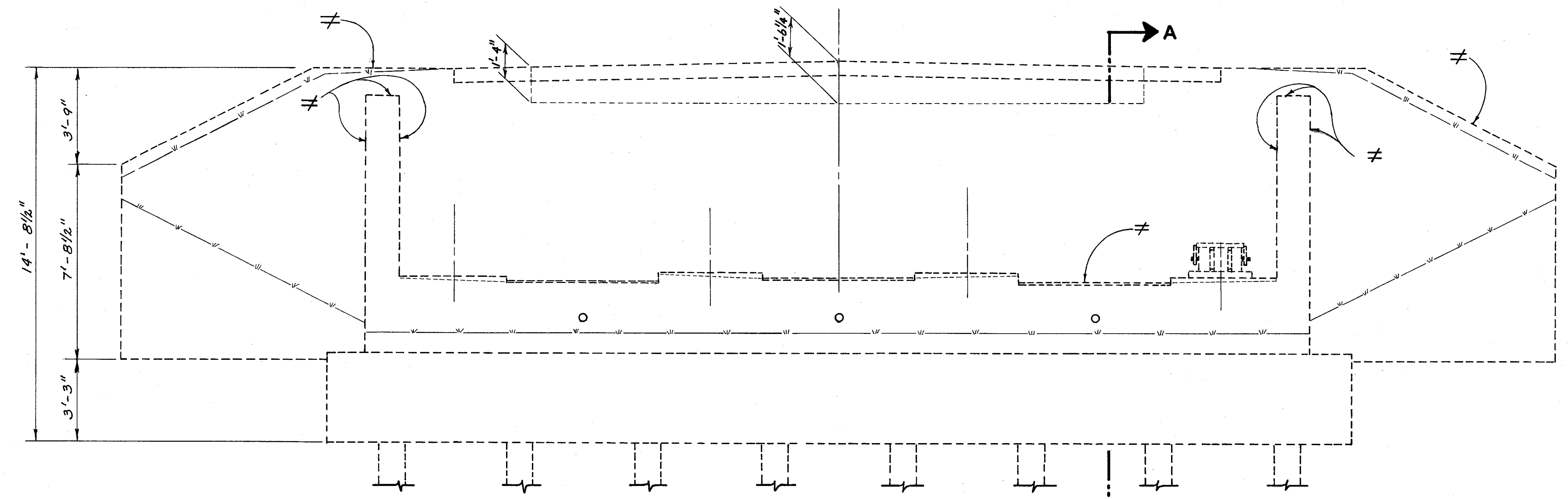
ELEVATION VIEW
