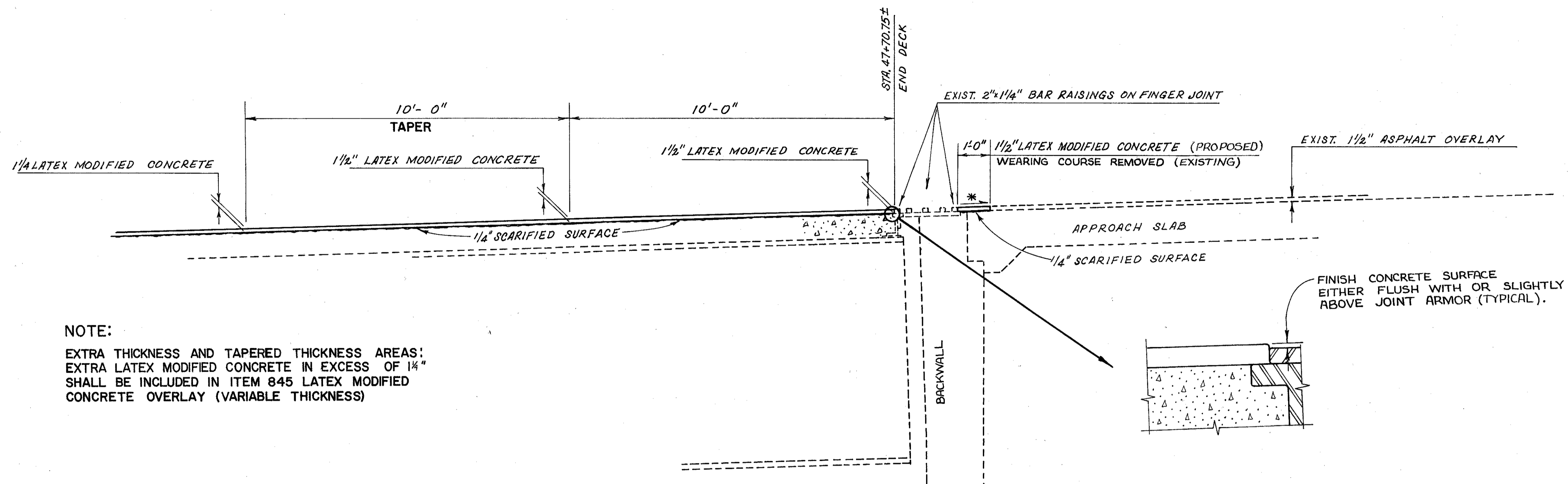
PAVEMENT FEATHER DETAIL NORTH END
