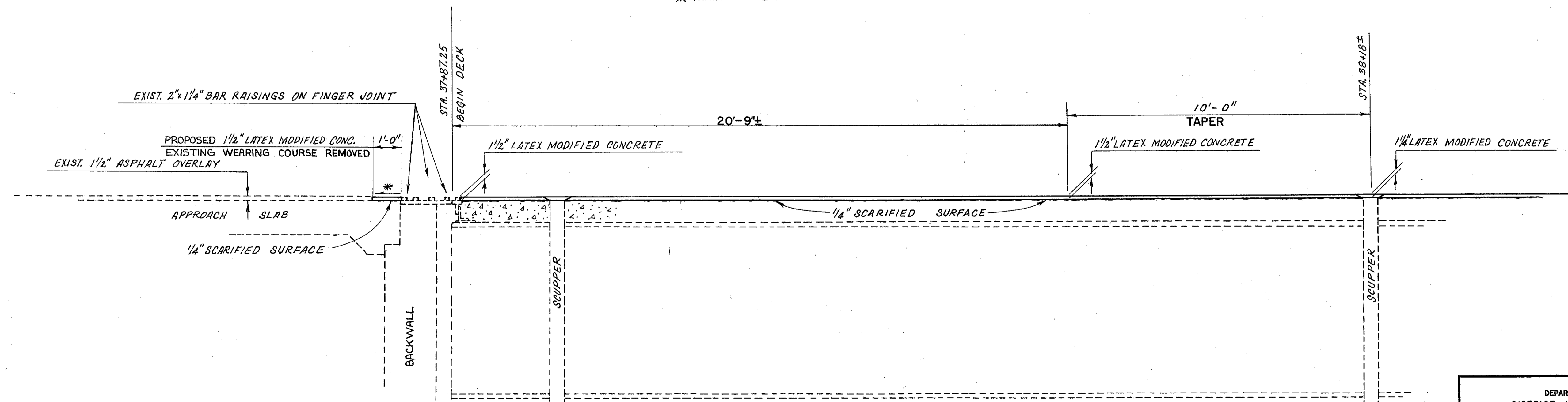
PAVEMENT FEATHER DETAIL SOUTH END
