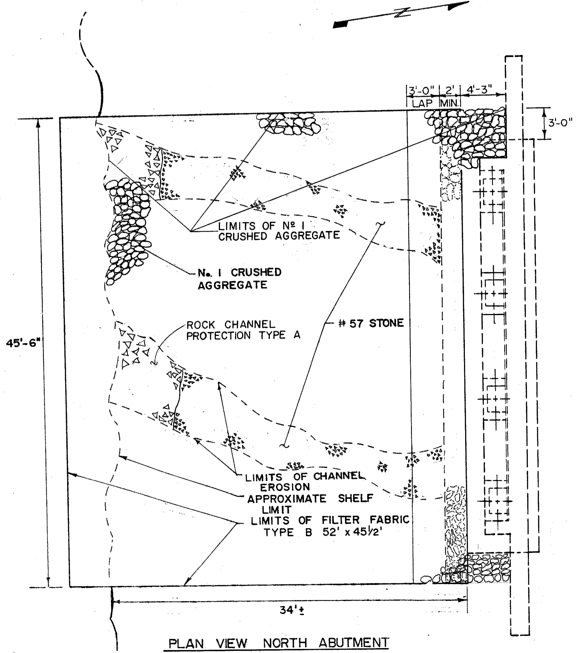
PLAN VIEW NORTH ABUTMENT
