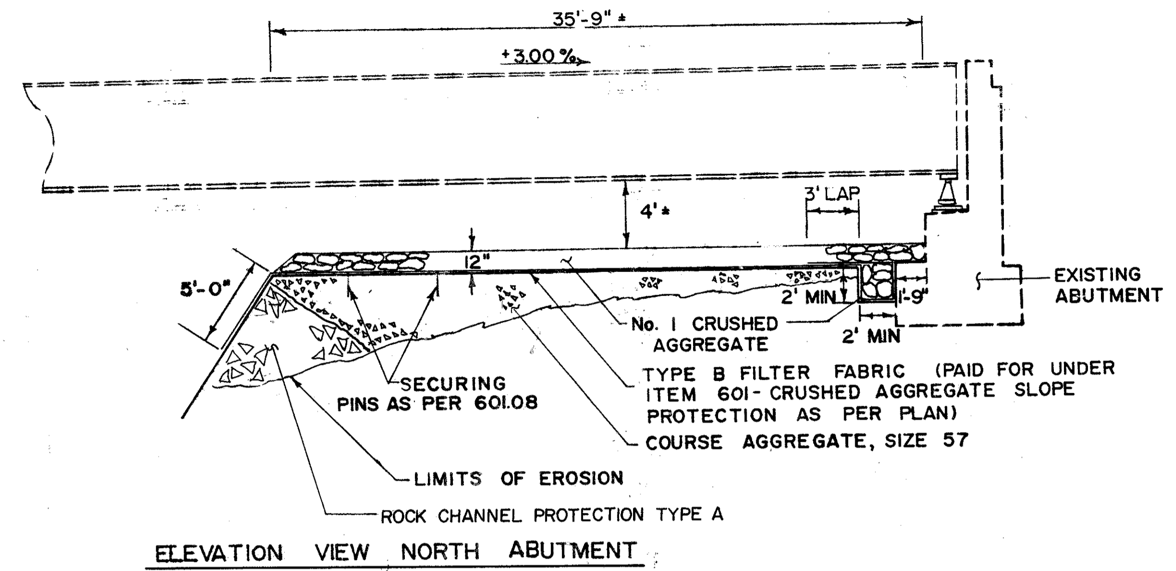
ELEVATION VIEW NORTH ABUTMENT
