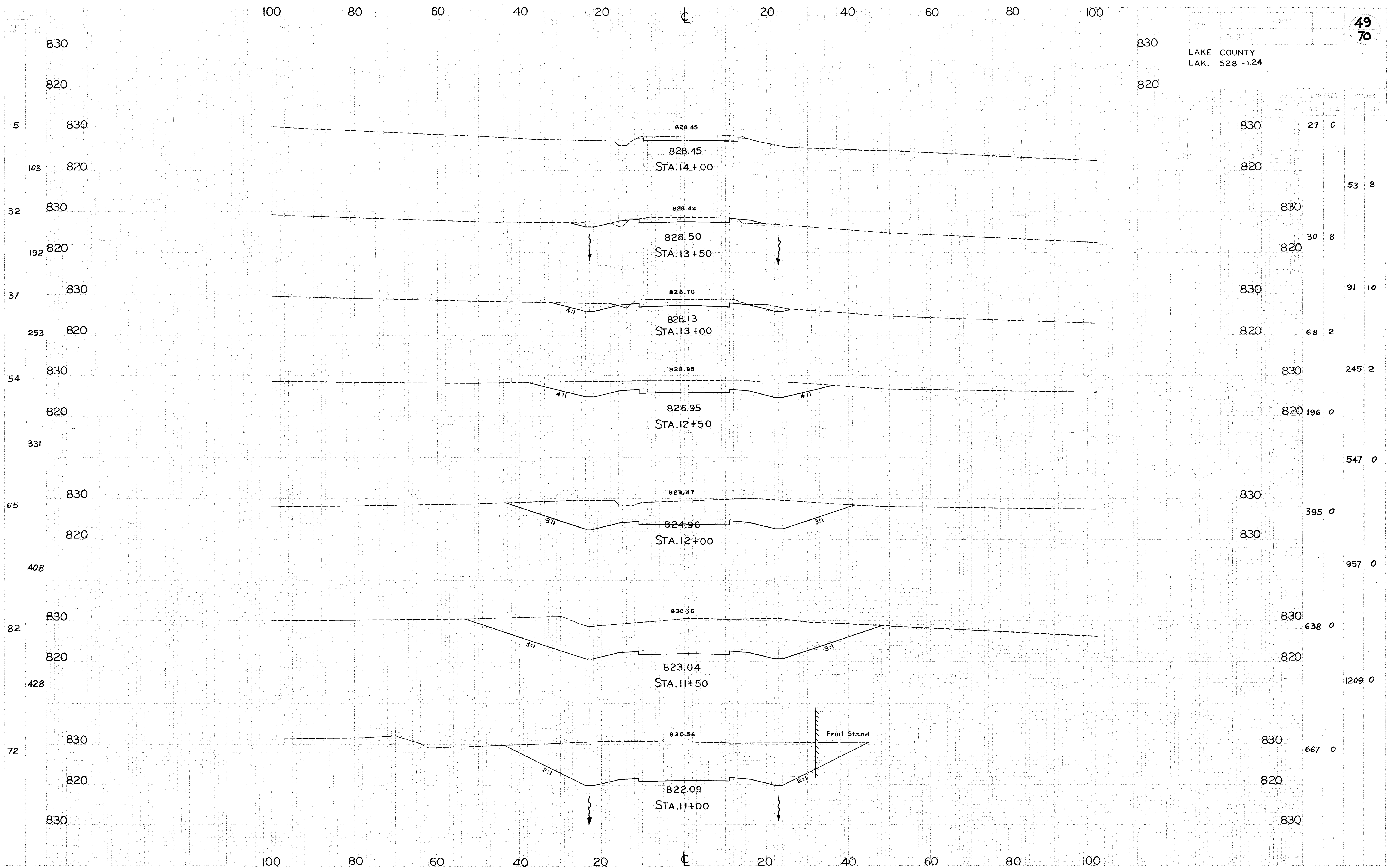
RIVER ROAD... CROSS SECTIONS... STA. 11+00 TO STA. 14+00
