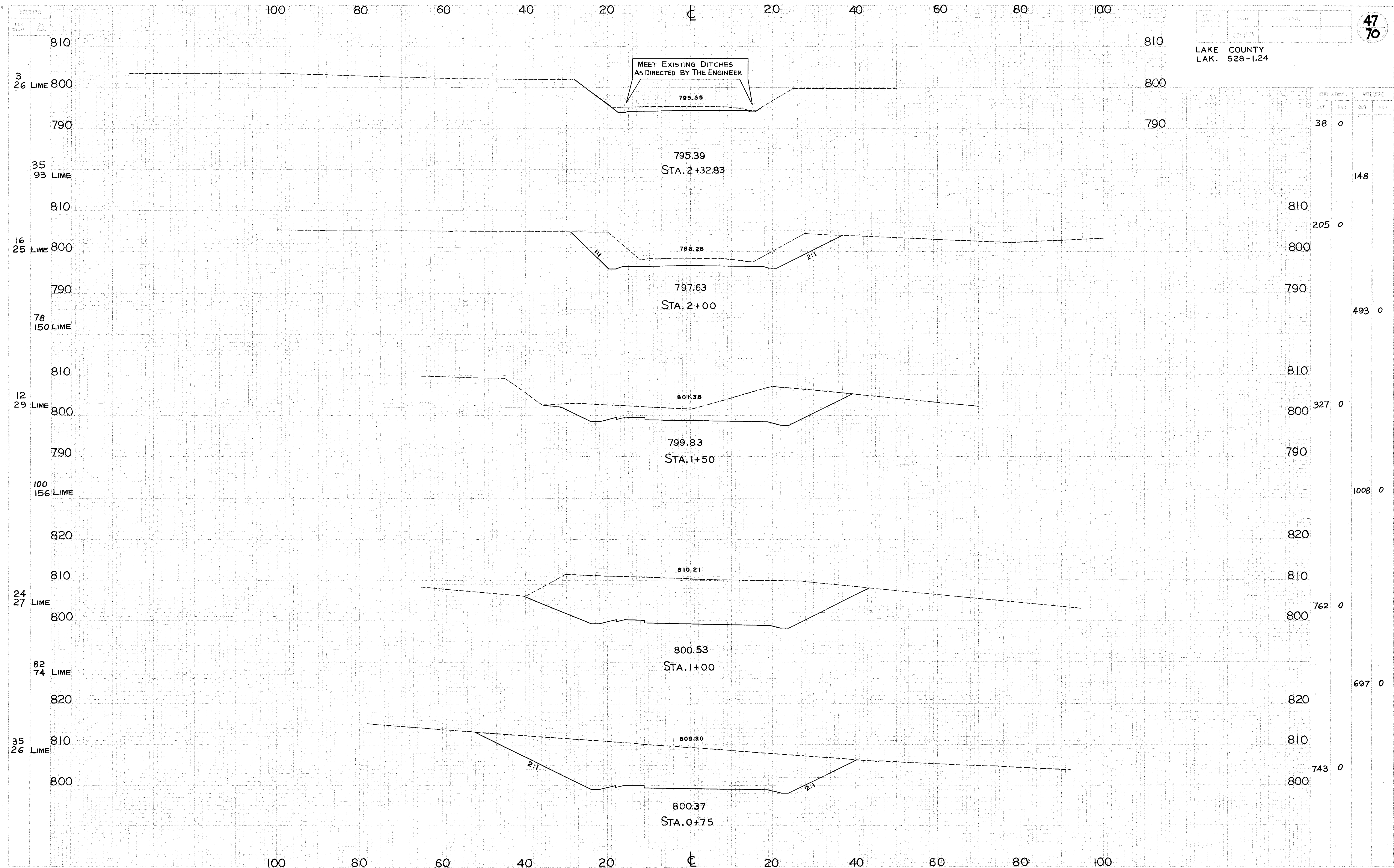
CONNECTING ROAD N° 2...CROSS SECTIONS STA. 0+75 TO STA. 2+32.87
