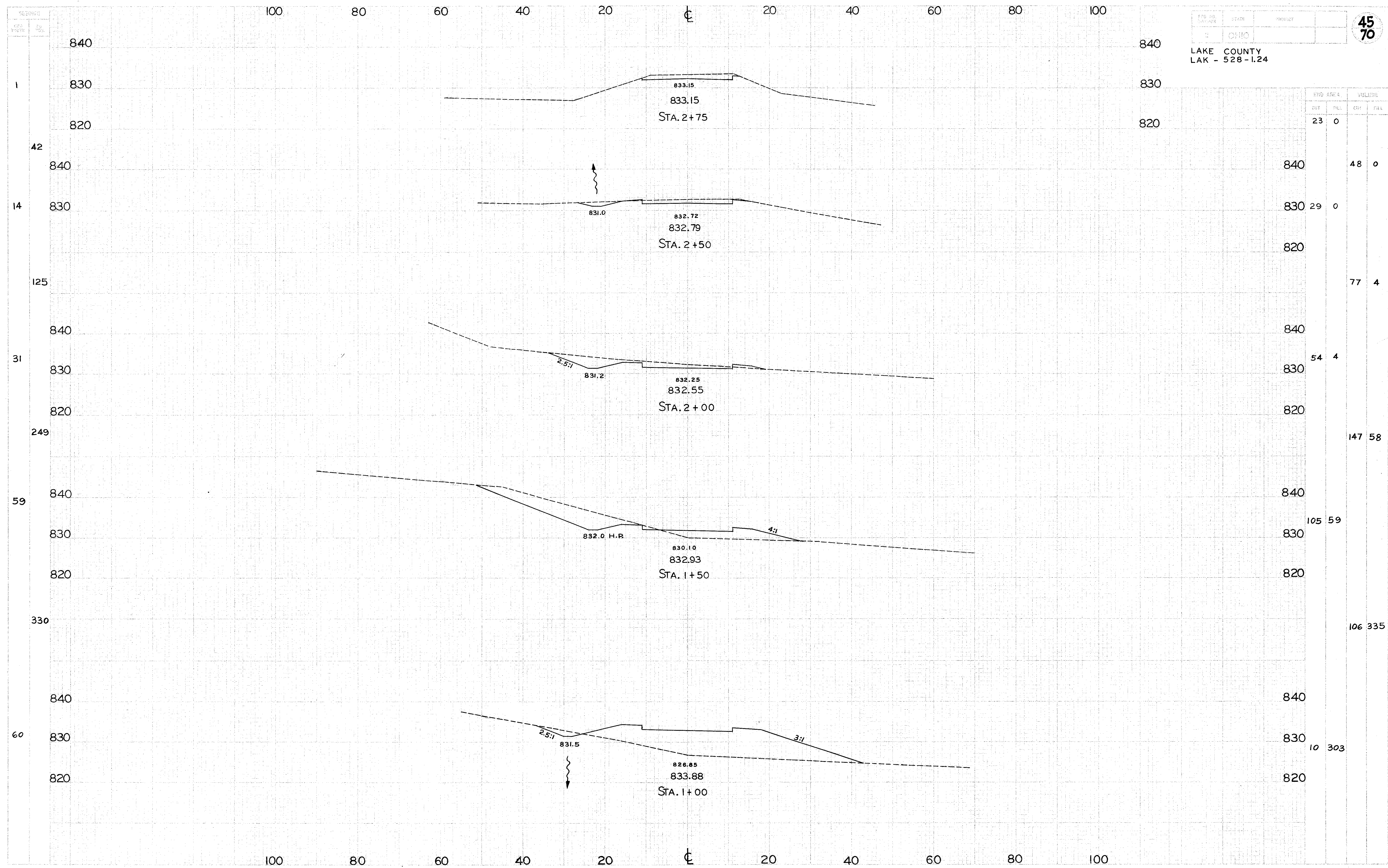
CONNECTING ROAD No. 1... CROSS SECTIONS STA. 1+00 TO STA. 2+75
