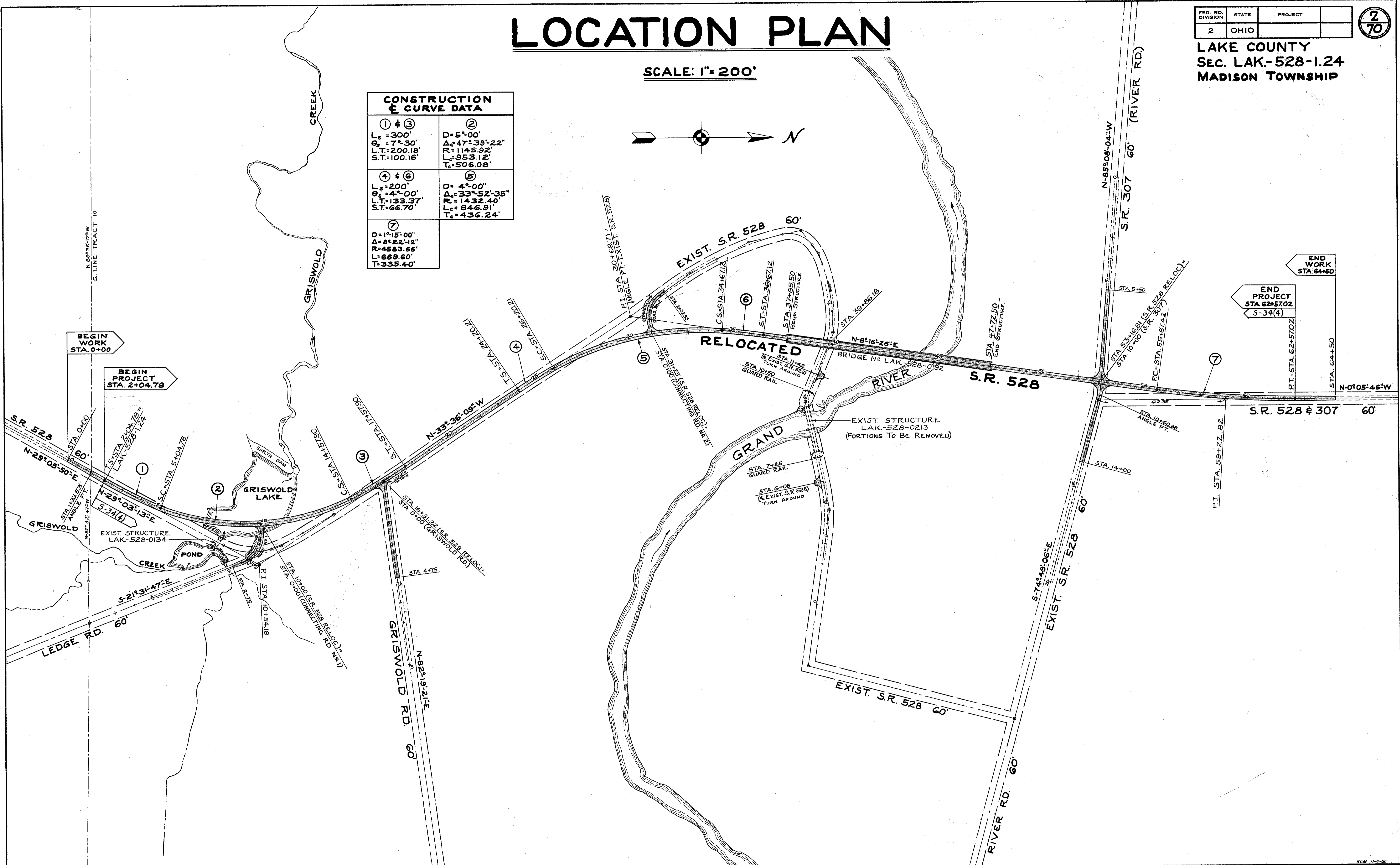
(S.R. No 528 RELOC.) LOCATION PLAN
