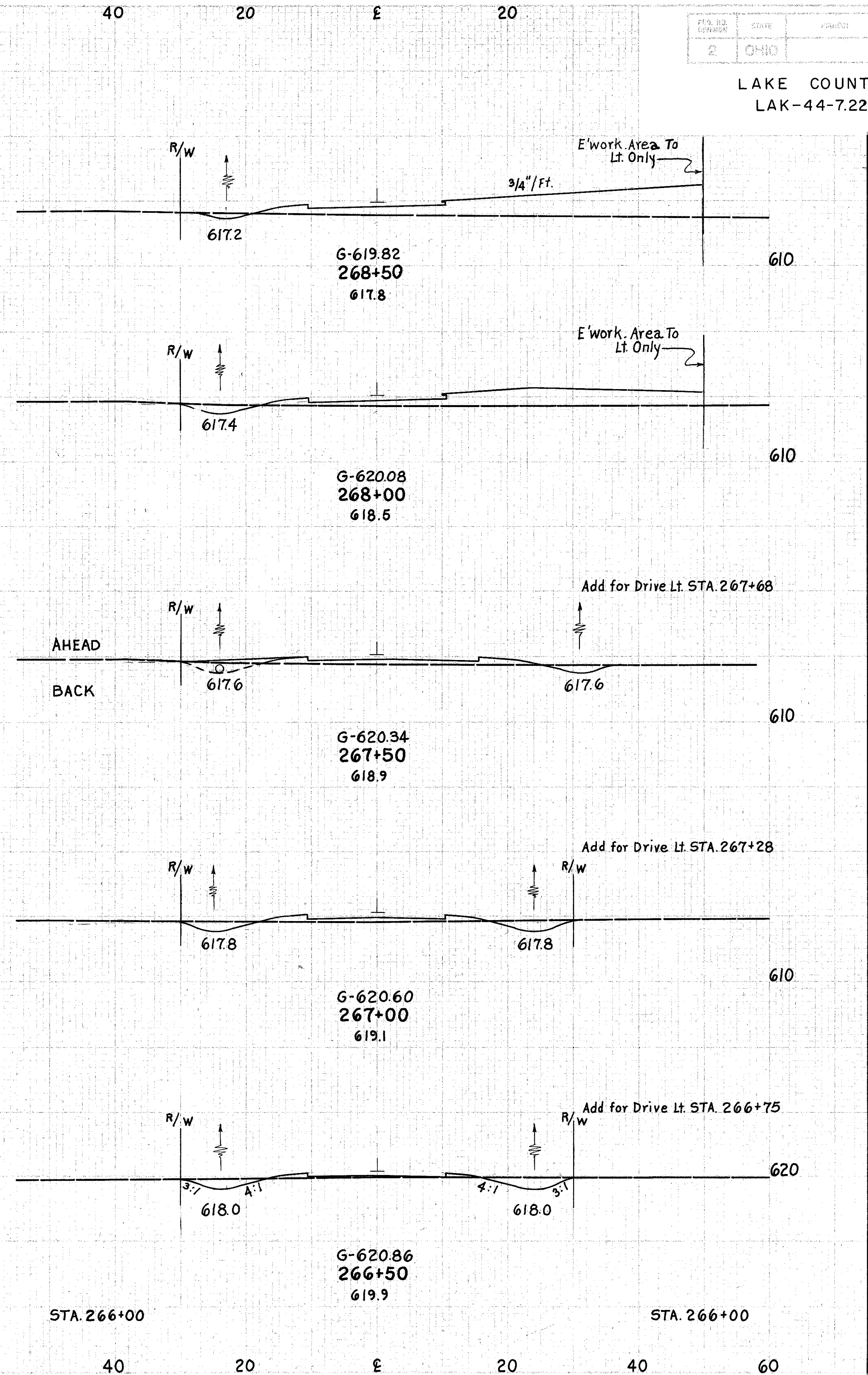
FRONTAGE ROAD, RIGHT Sta. 264+00 to 268+50
