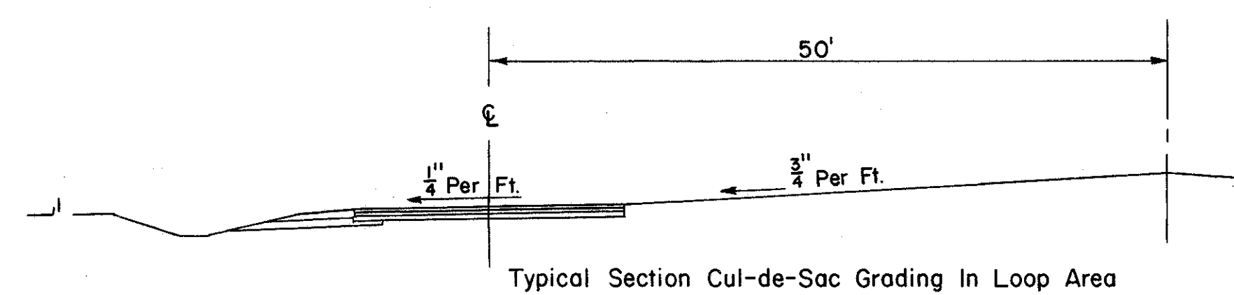
Typical Section Cul-de-Sac Grading In Loop Area
