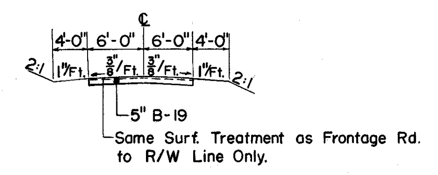
TYPICAL SECTION DRIVES
