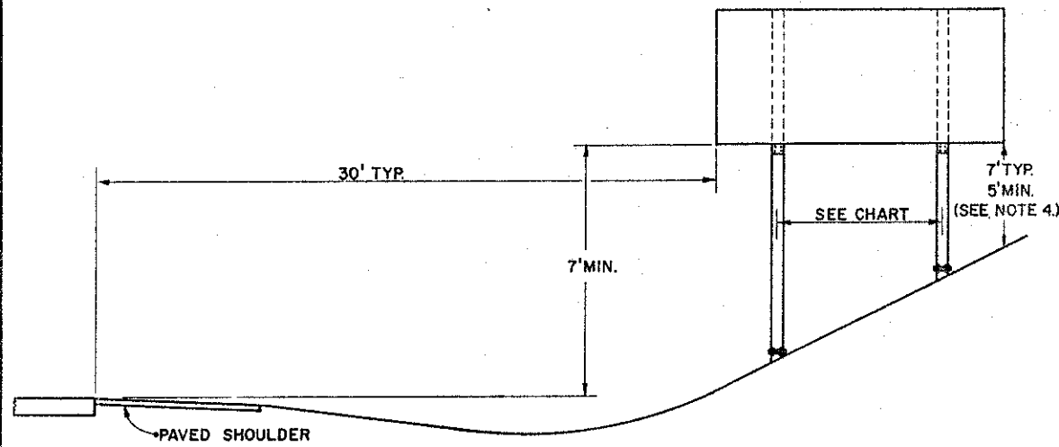
TYPICAL INSTALLATION, CUT SECTION, 30' OFFSET
