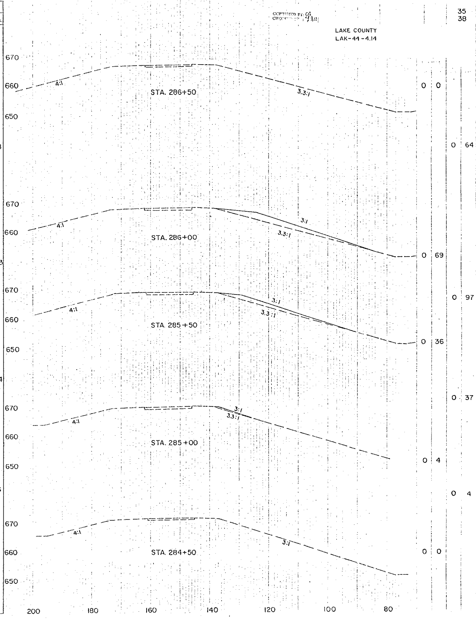
RAMP NO. 1 STA. 284+50 TO 286+50 (LEFT SIDE)
