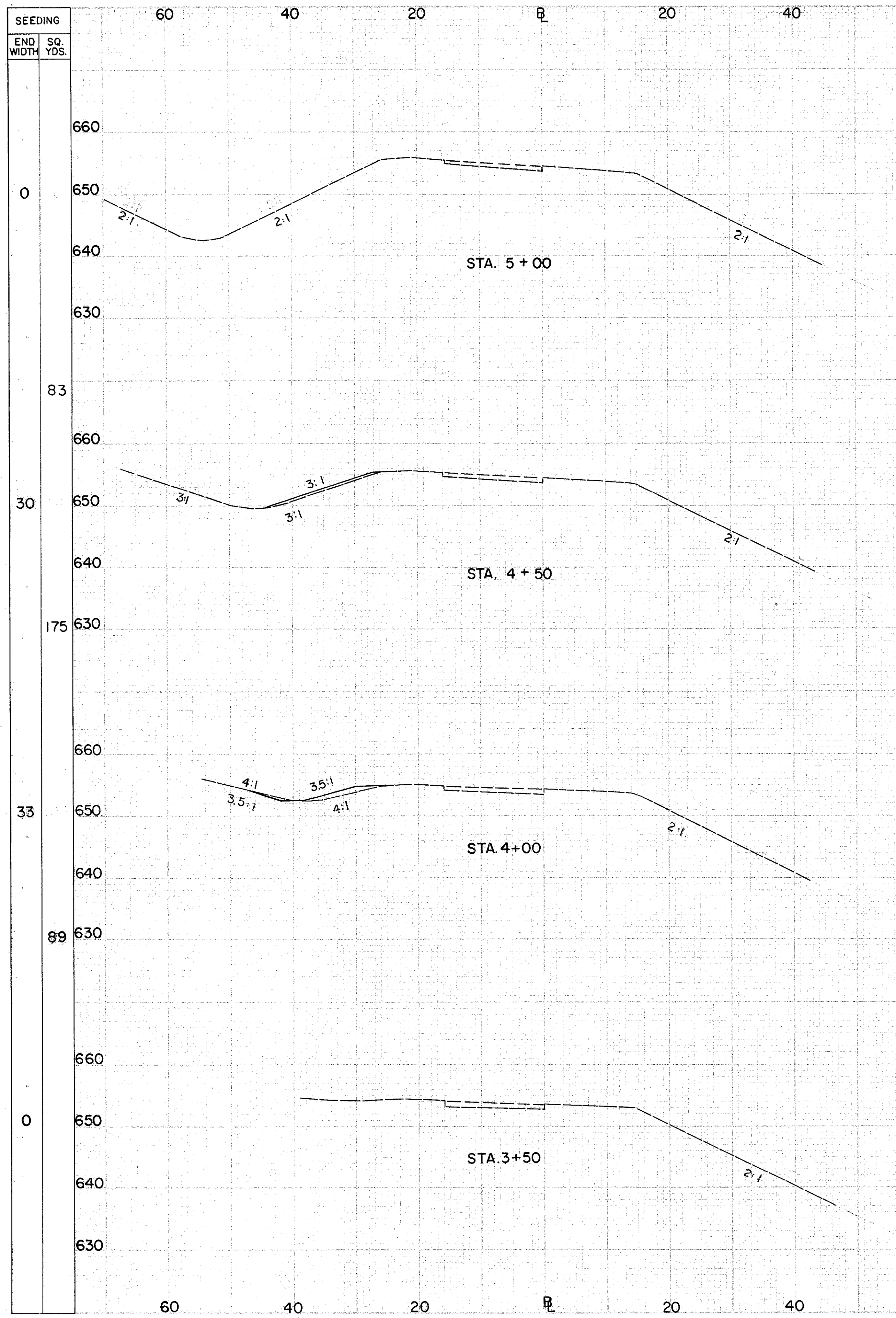
RAMP H 3+50 TO 5+00
