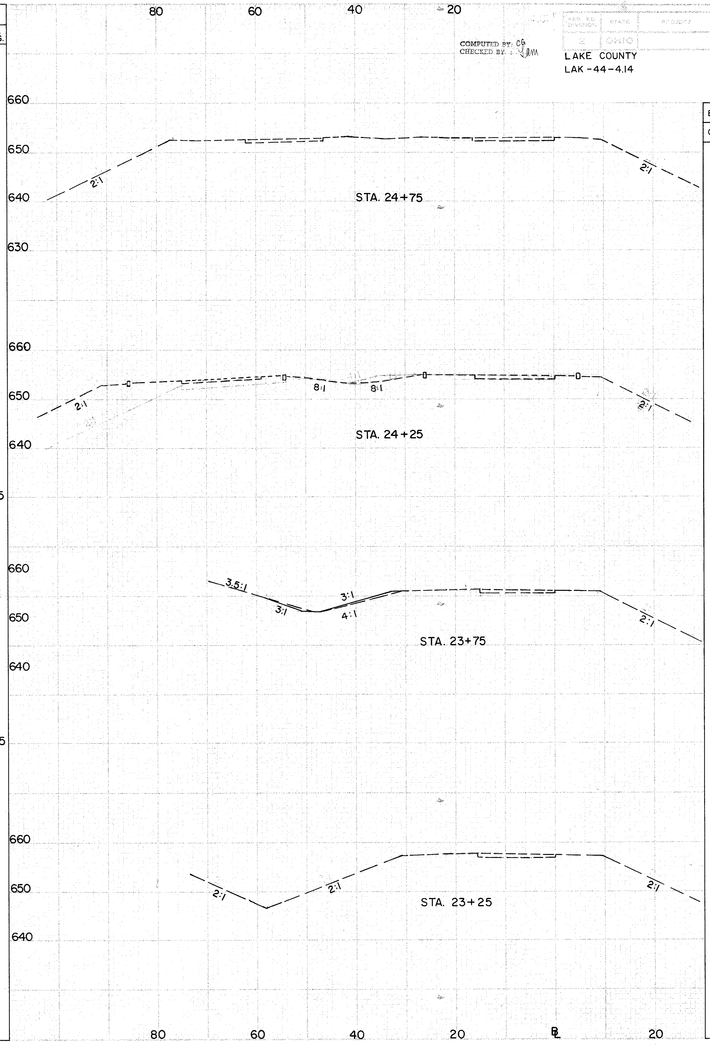
RAMP E 23+25 TO 24+75
