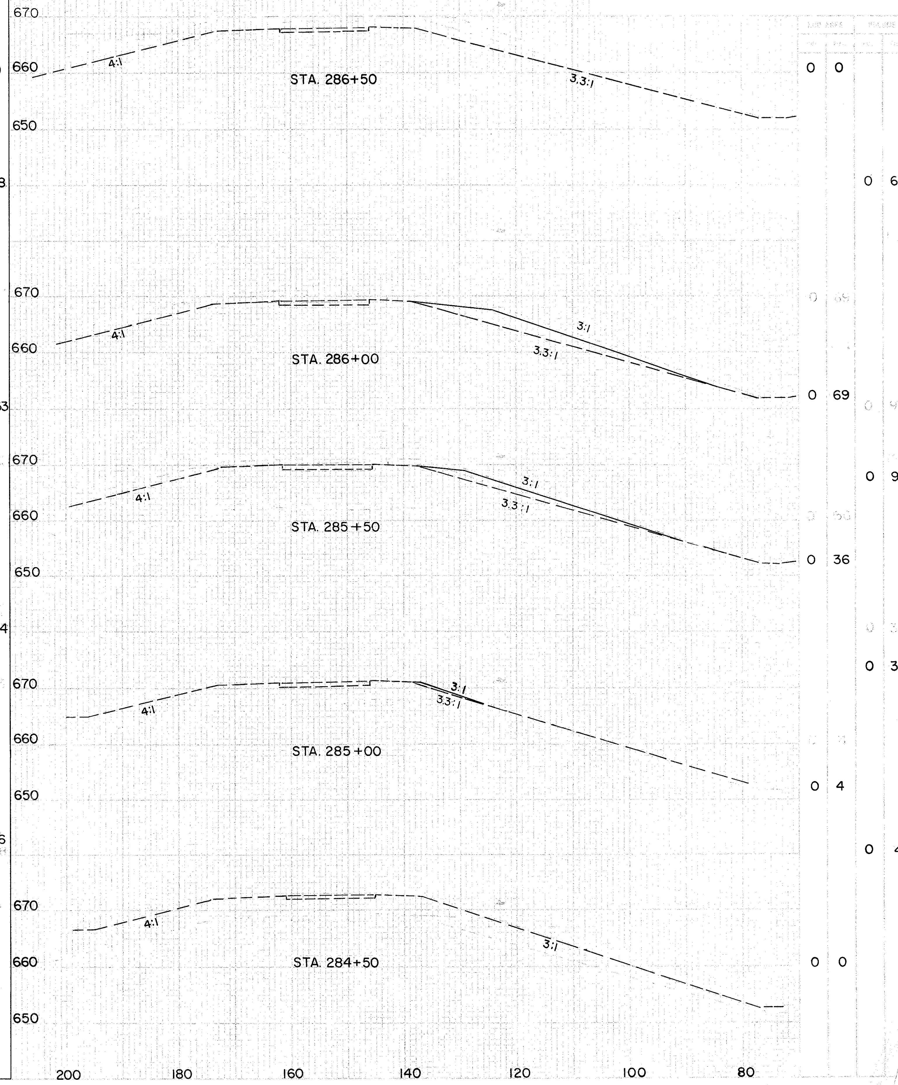
RAMP NO. 1 STA. 284+50 TO 286+50 (LEFT SIDE)
