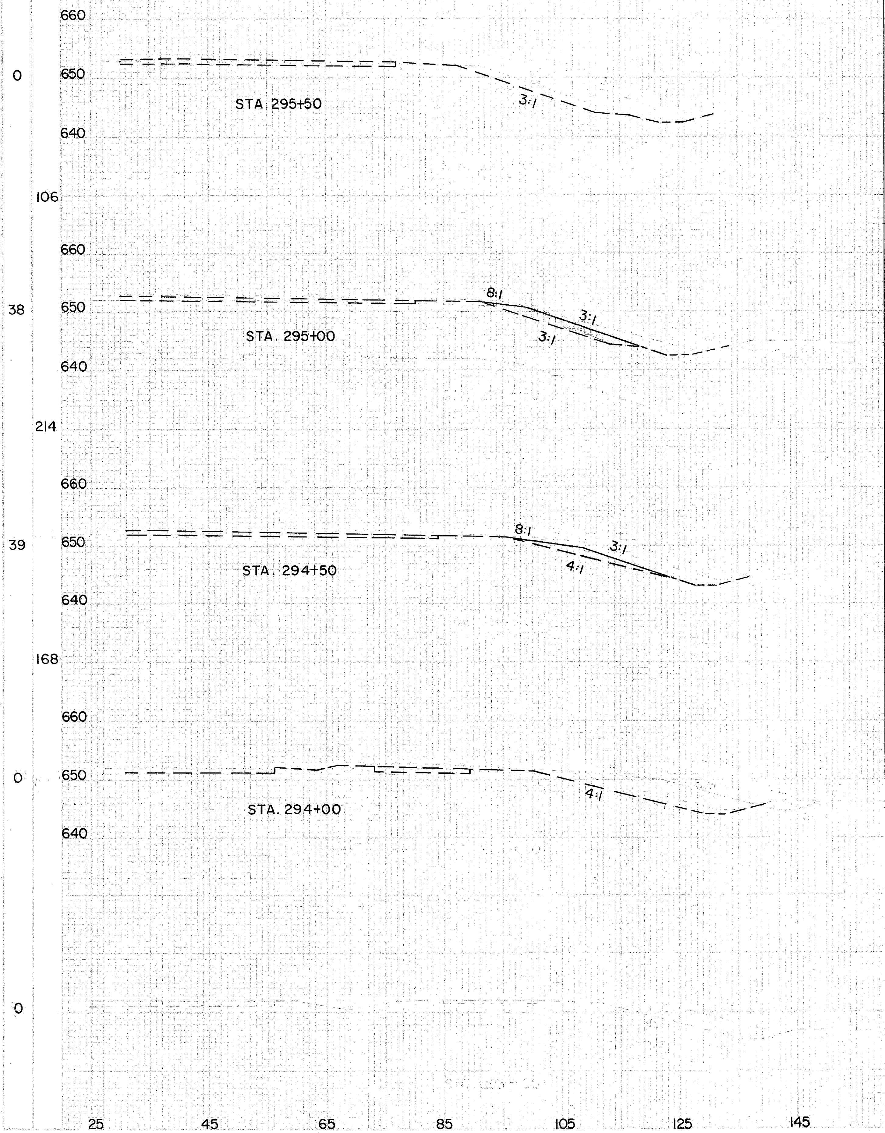
RAMP NO. 2 STA. 294+00 TO 295+50 (RIGHT SIDE)
