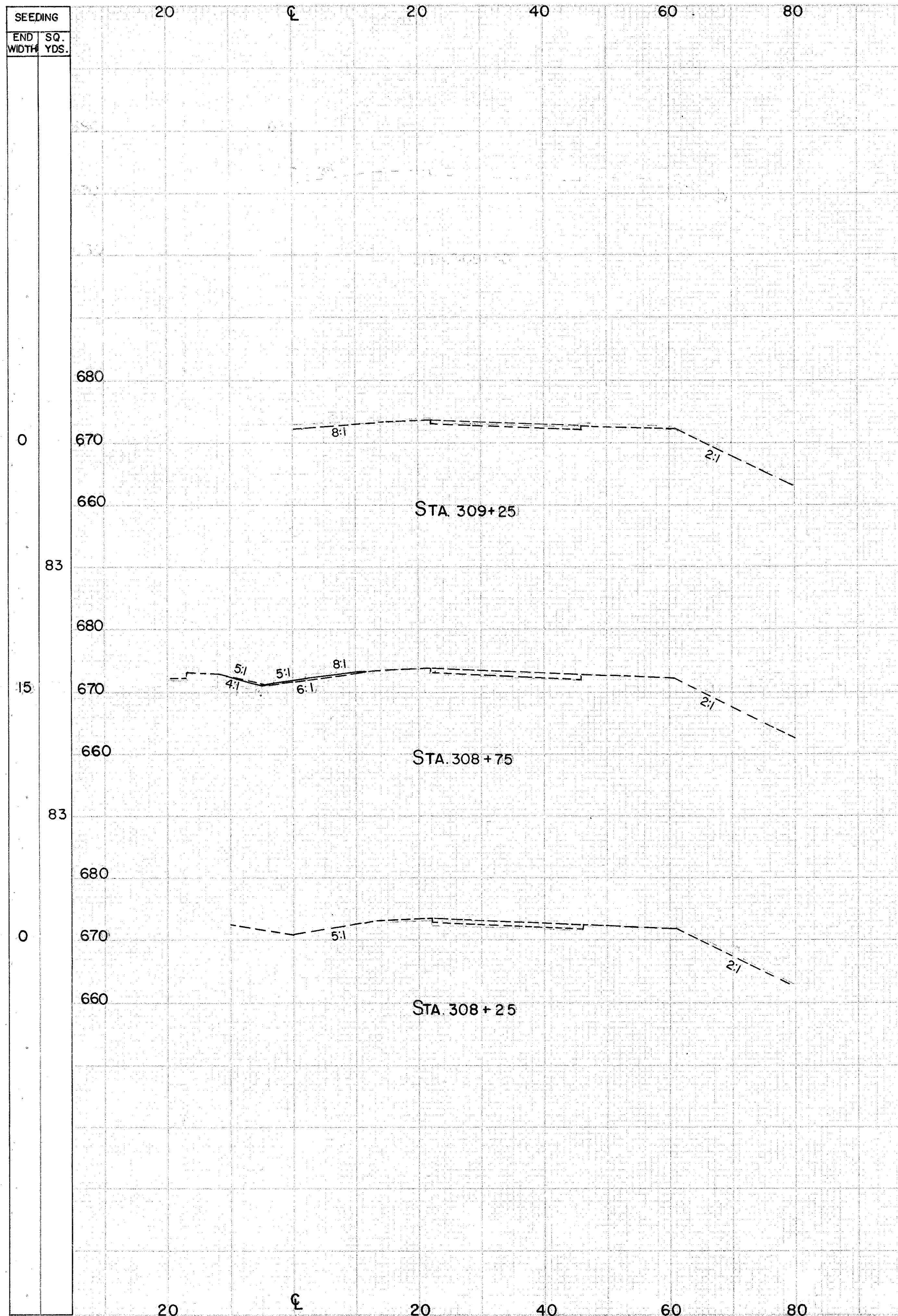
STA. 308+25 TO 309+25 (LEFT SIDE)
