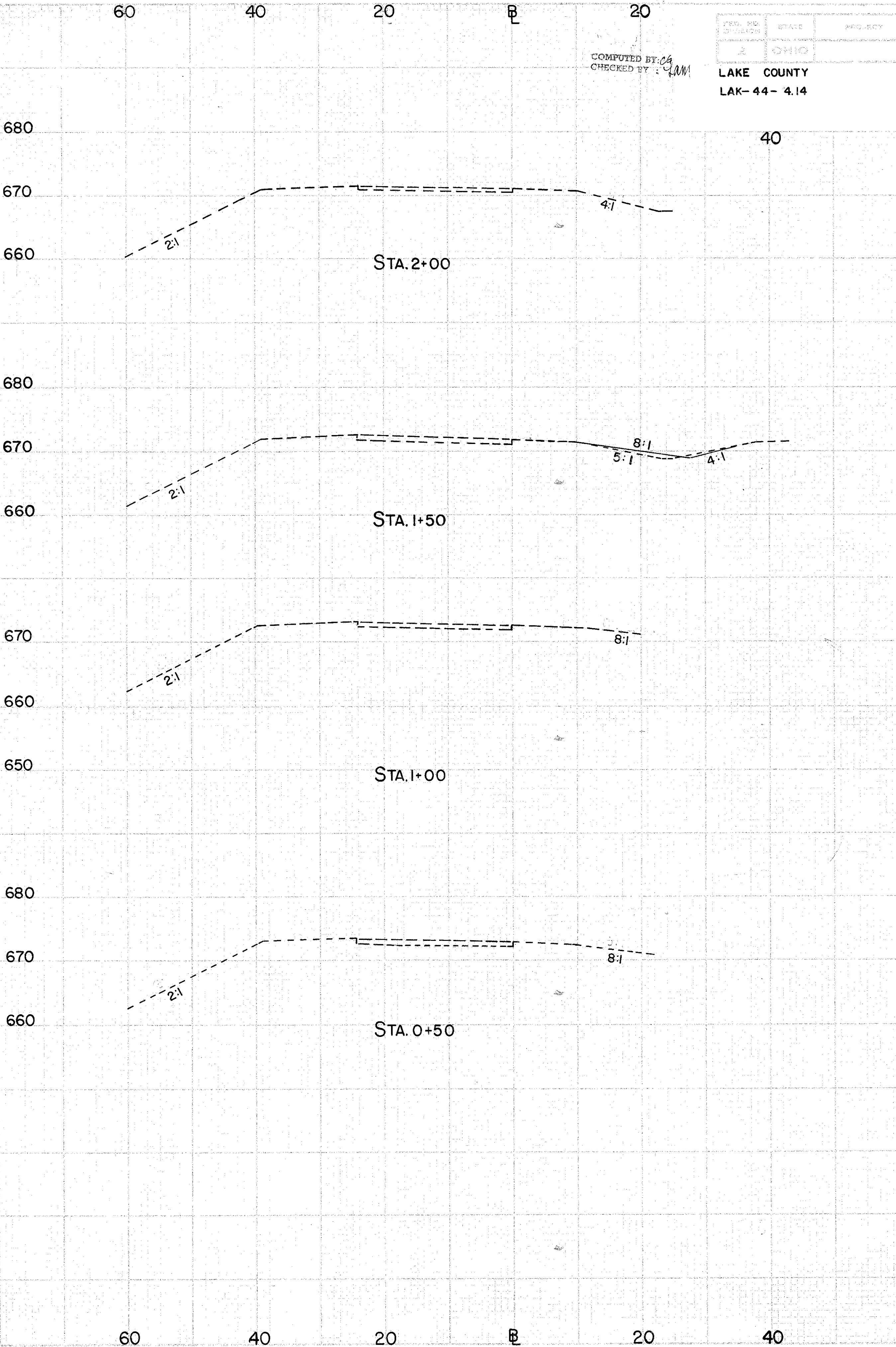
RAMP G STA. 0+50 TO 2+00 (LEFT SIDE)
