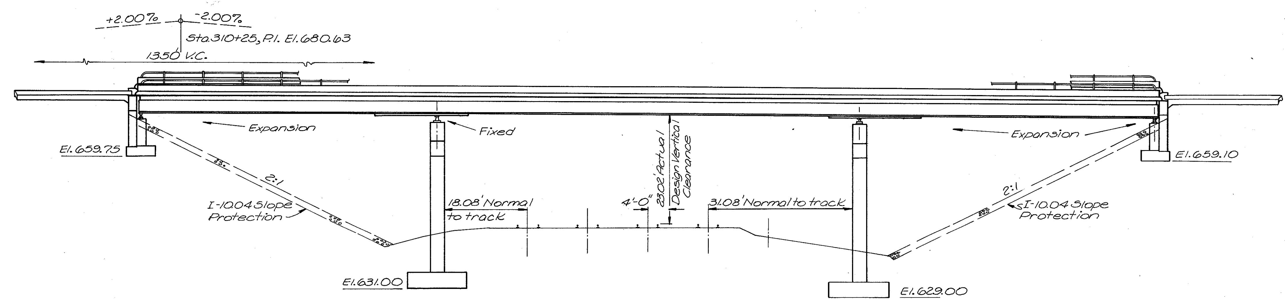
ELEVATION (Northbound bridge shown)
