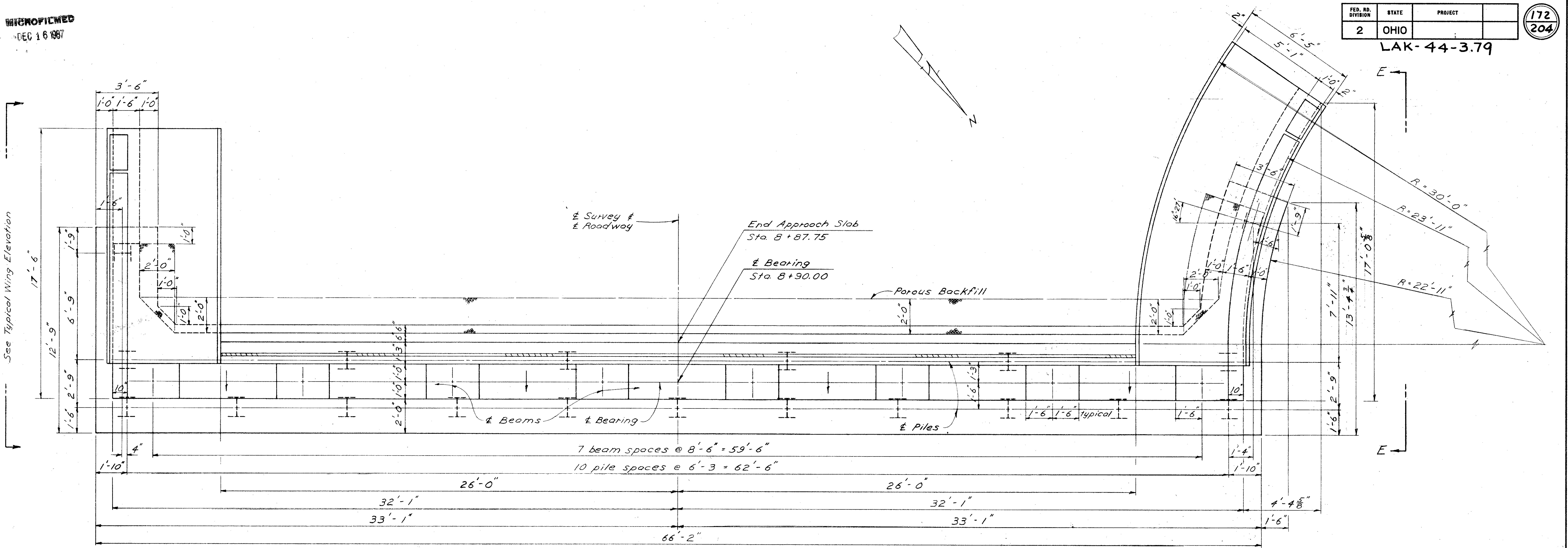
PLAN
