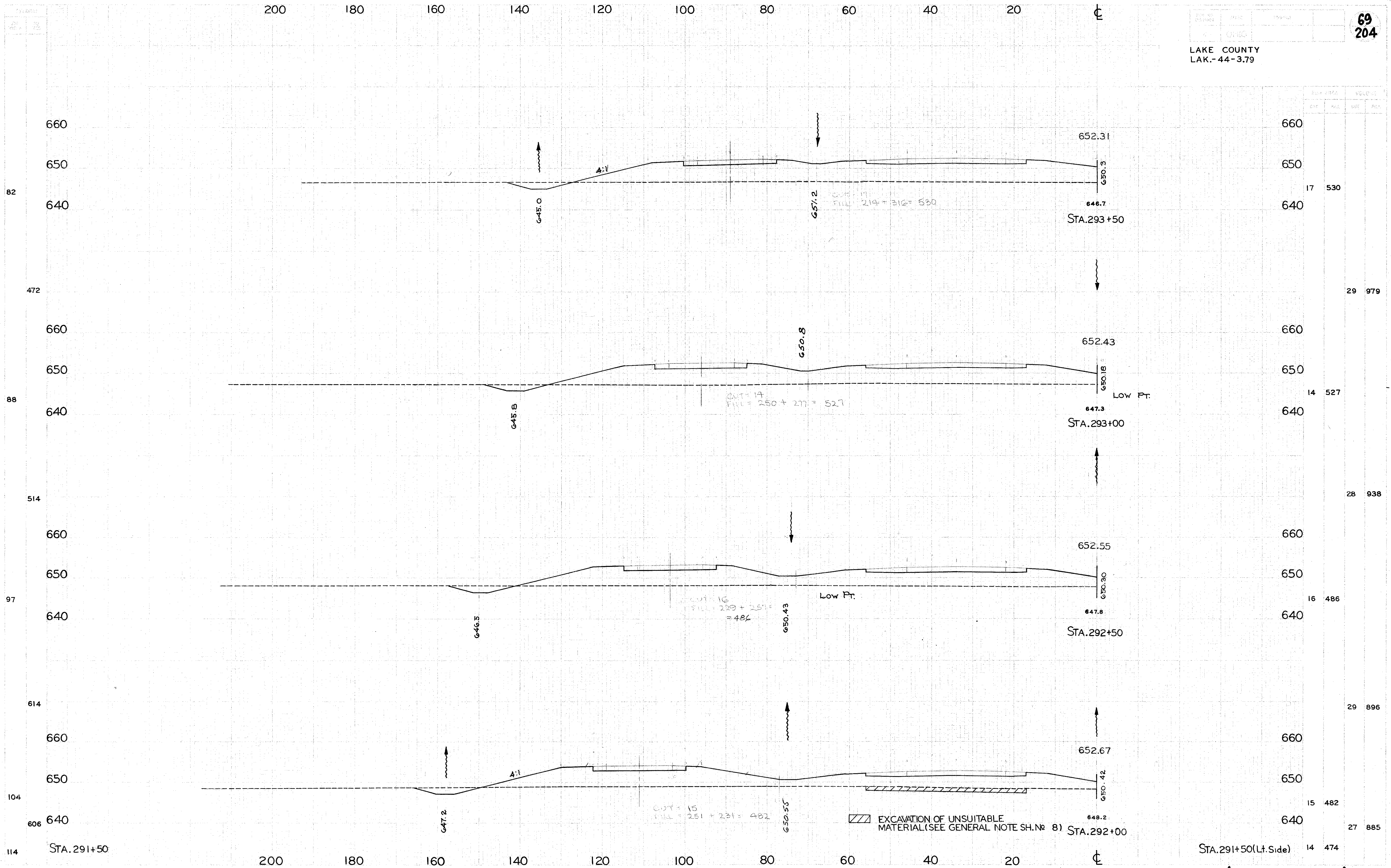
CROSS SECTIONS STA.292+00 TO STA.293+50 (LEFT SIDE)
