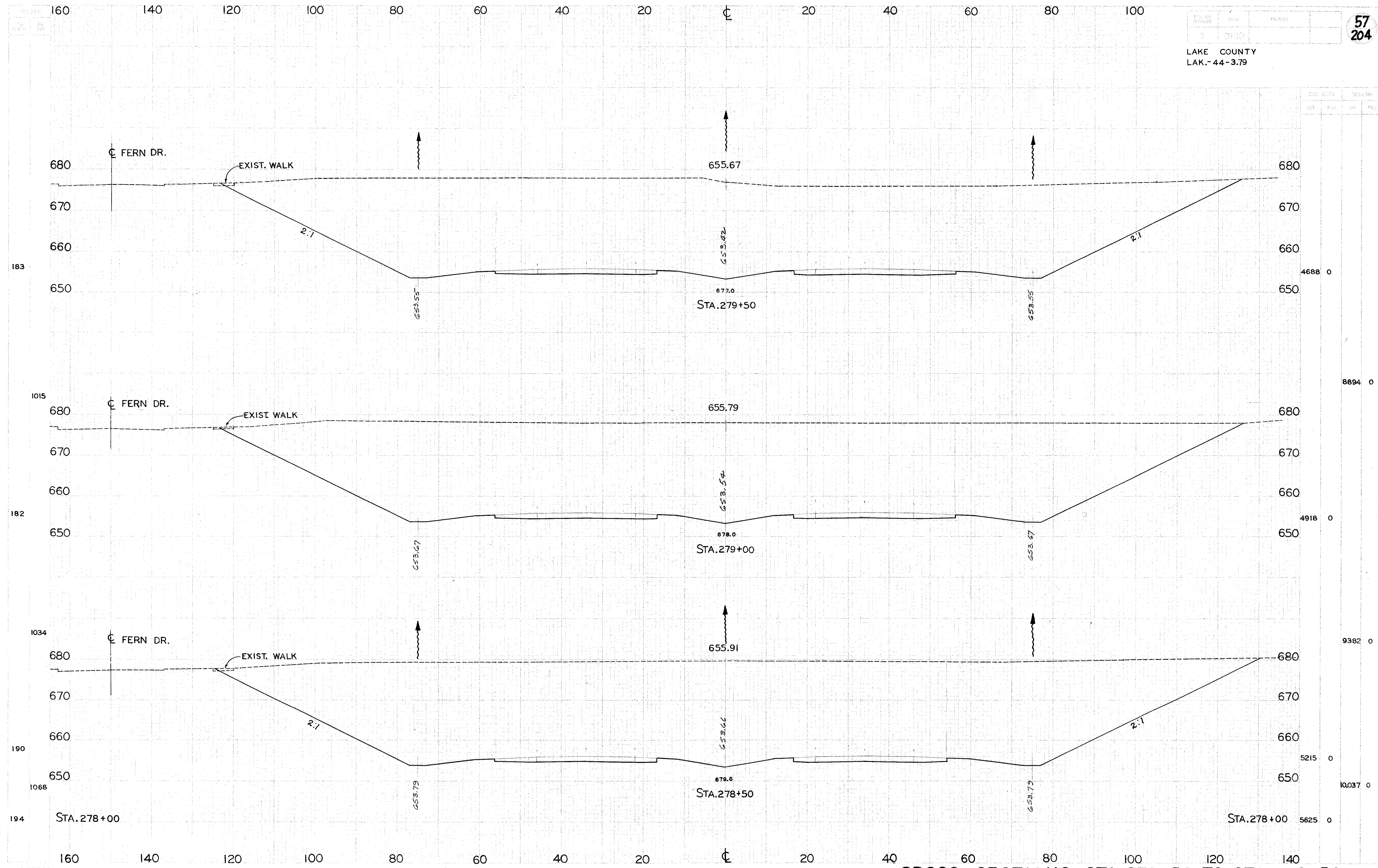
CROSS SECTIONS STA.278+50 TO STA.279+50
