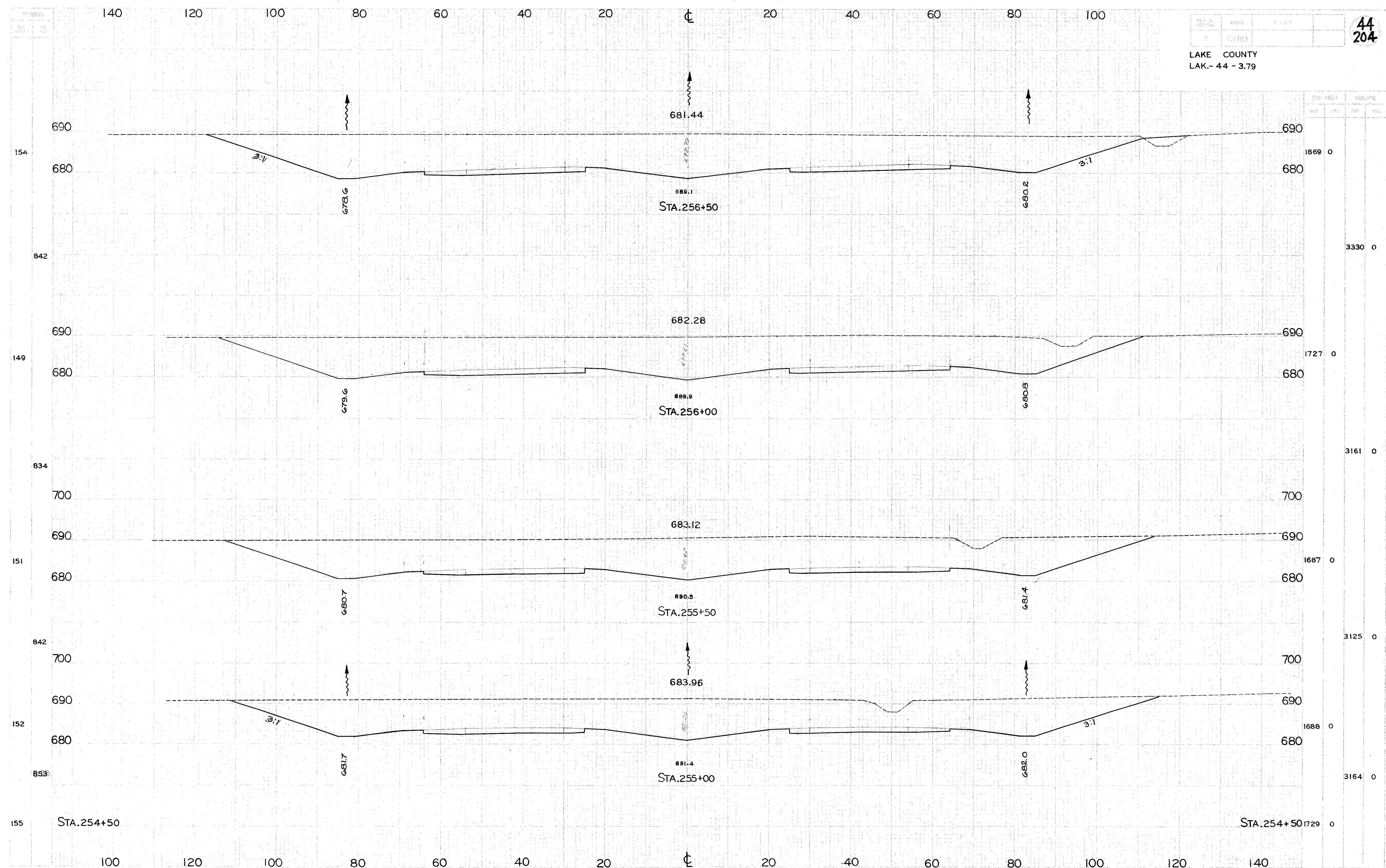
CROSS SECTIONS STA.255+00 TO STA.256+50
