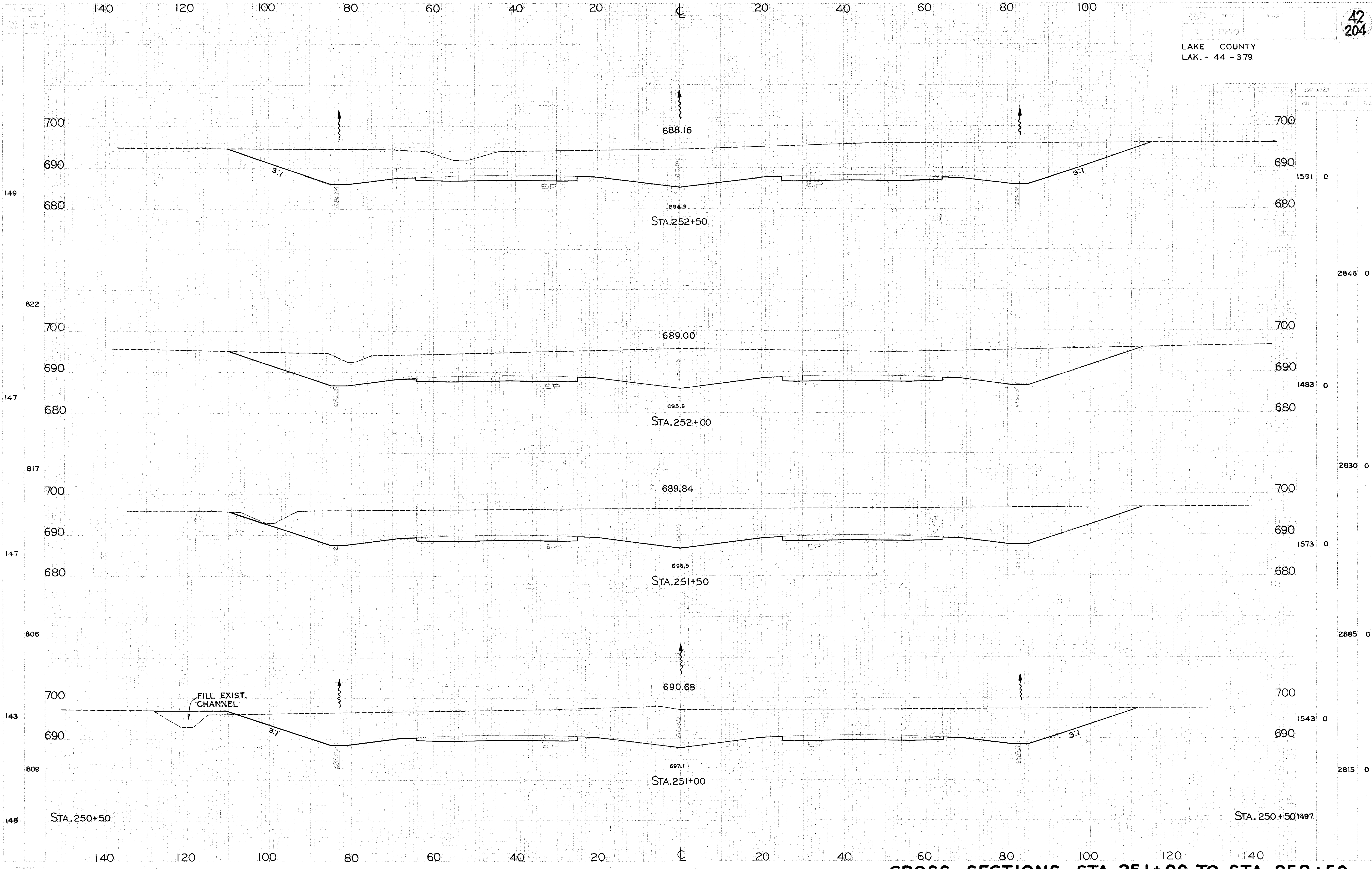
CROSS SECTIONS STA.251+00 TO STA.252+50
