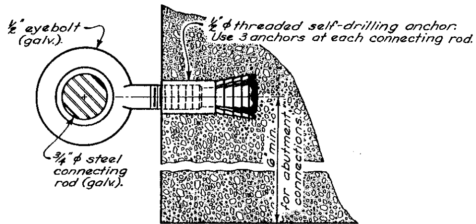
ABUTMENT CONNECTION
