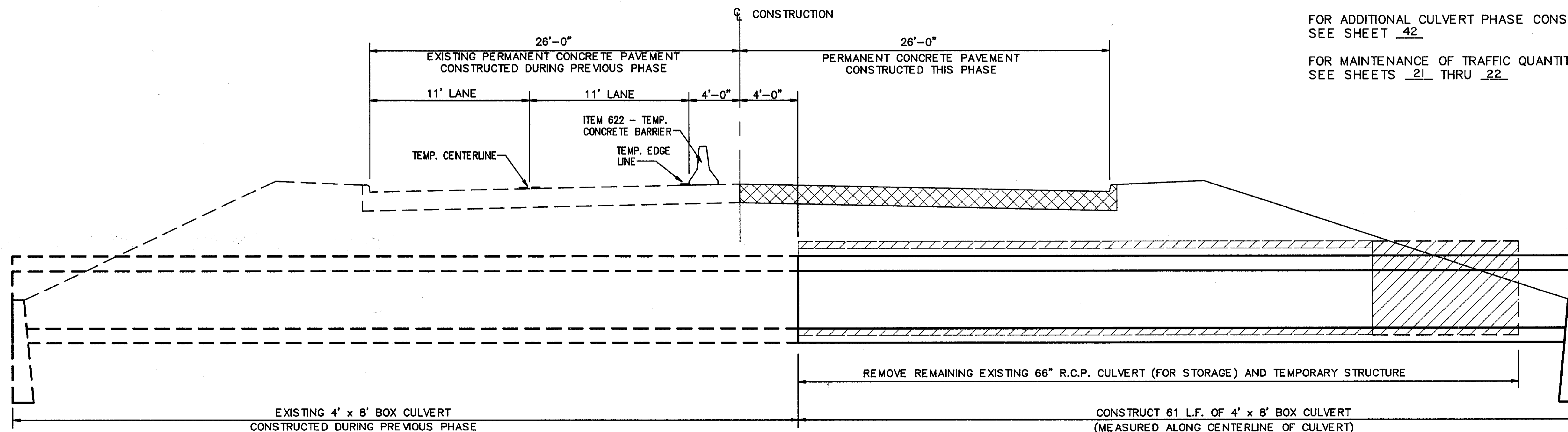
TYPICAL SECTION - SECTION 3 PHASE B (NO SCALE)
