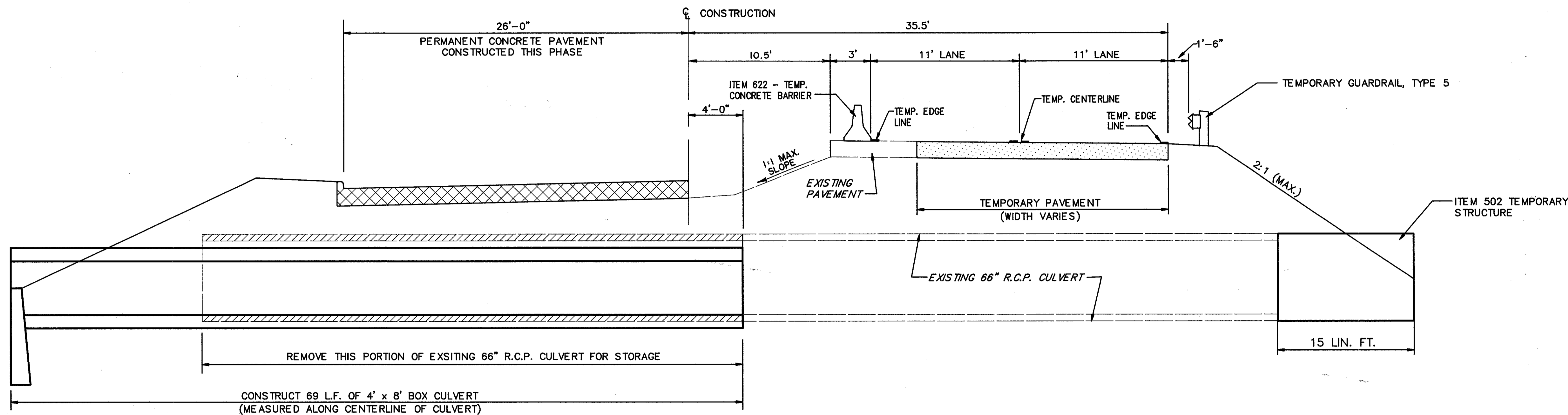
TYPICAL SECTION - SECTION 3 PHASE A (NO SCALE)
