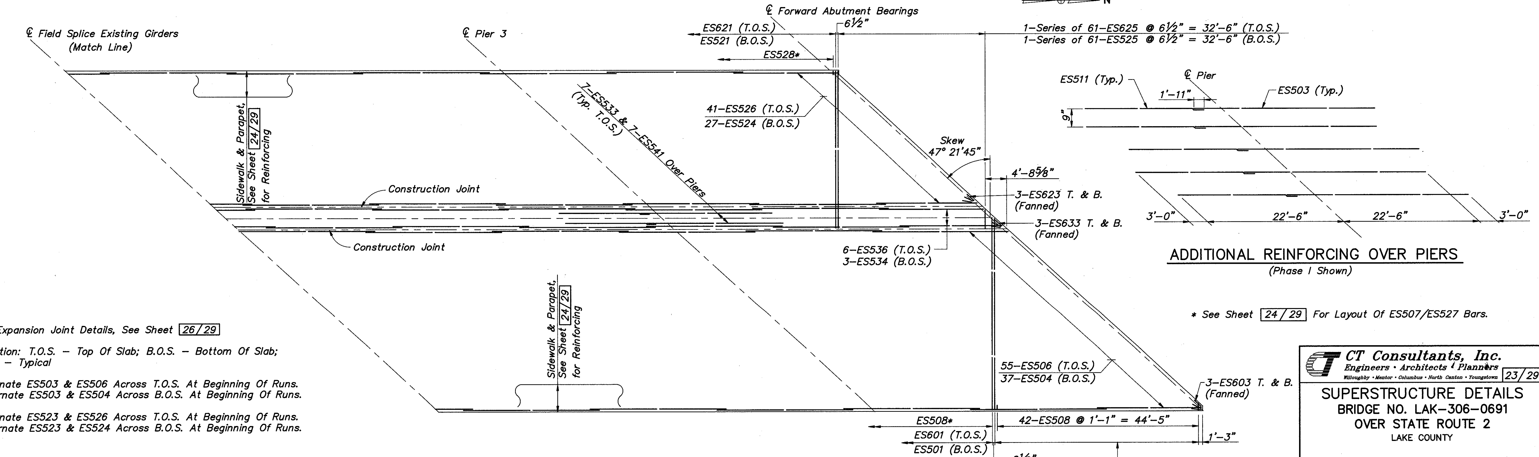
SLAB REINFORCING PLAN
