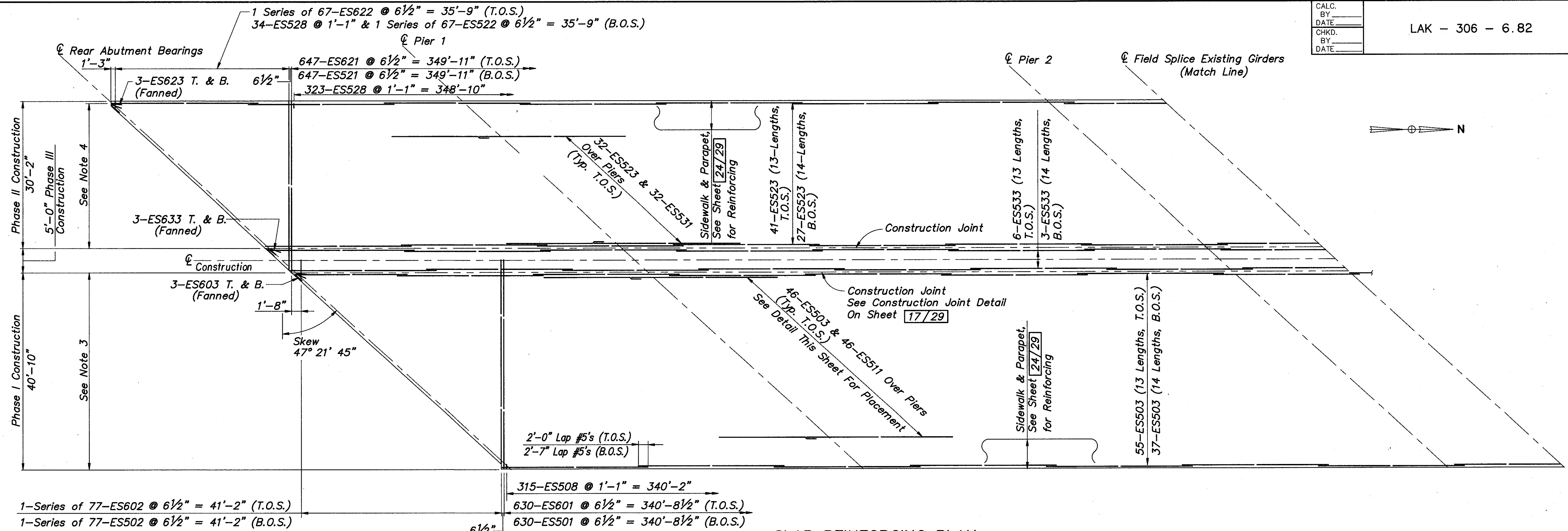
SLAB REINFORCING PLAN
