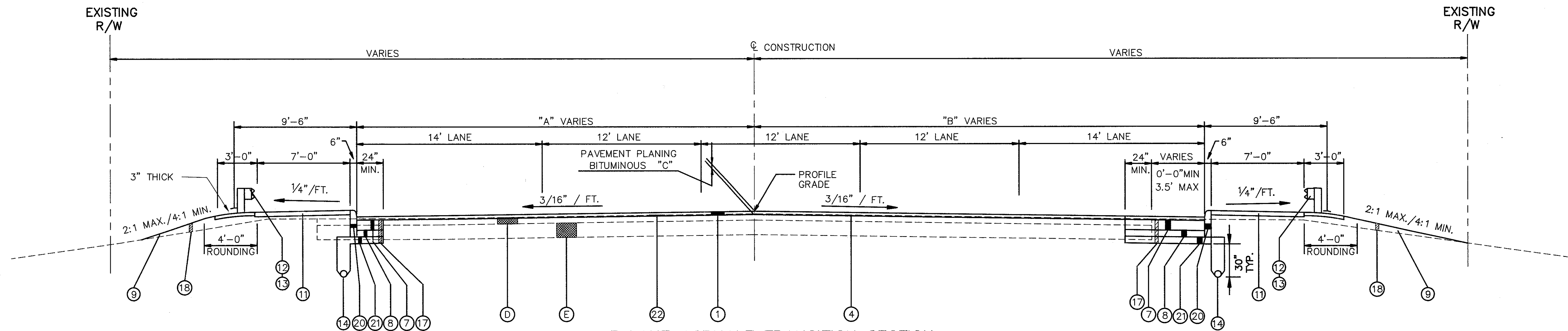
5 LANE ASPHALT TRANSITION SECTION STA. 35+50.00 TO STA. 38+30.00 = 280.00 LIN. FT.
