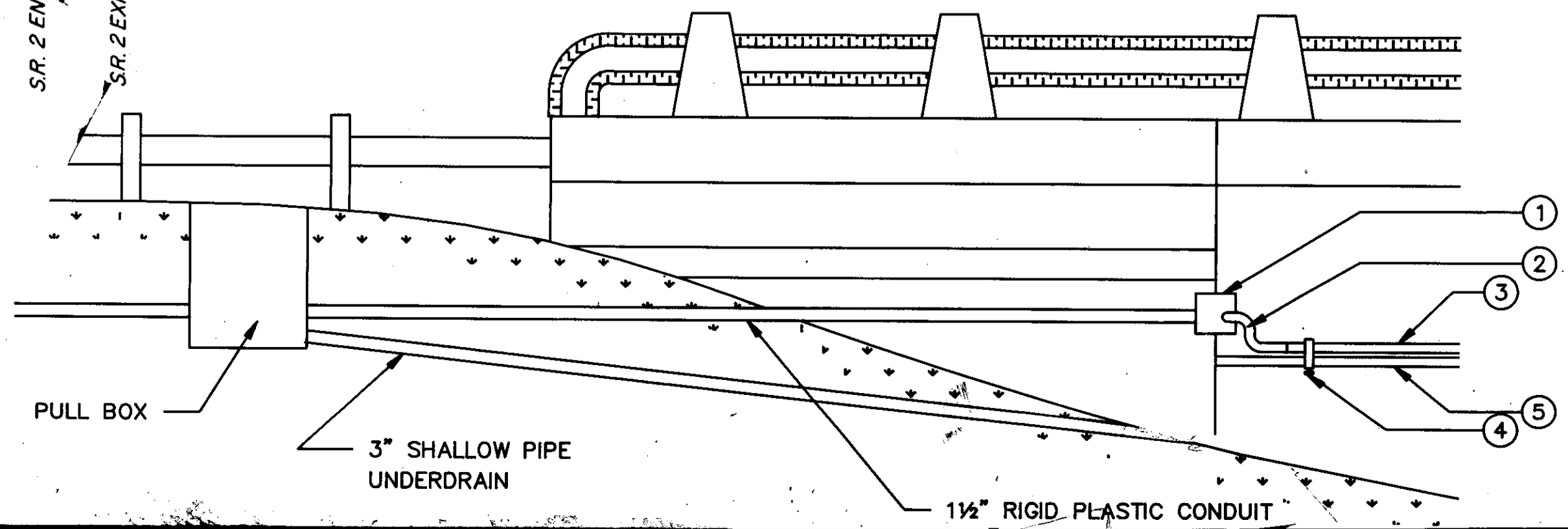
SCHMATIC FOR INTERCONNECT BRIDGE CONNECTION SKETCH NOT TO SCALE
