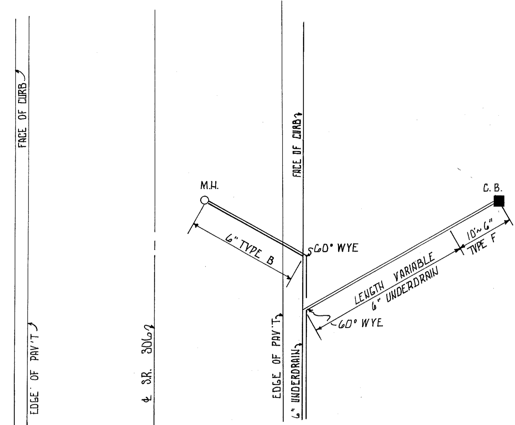
DETAIL "B"
