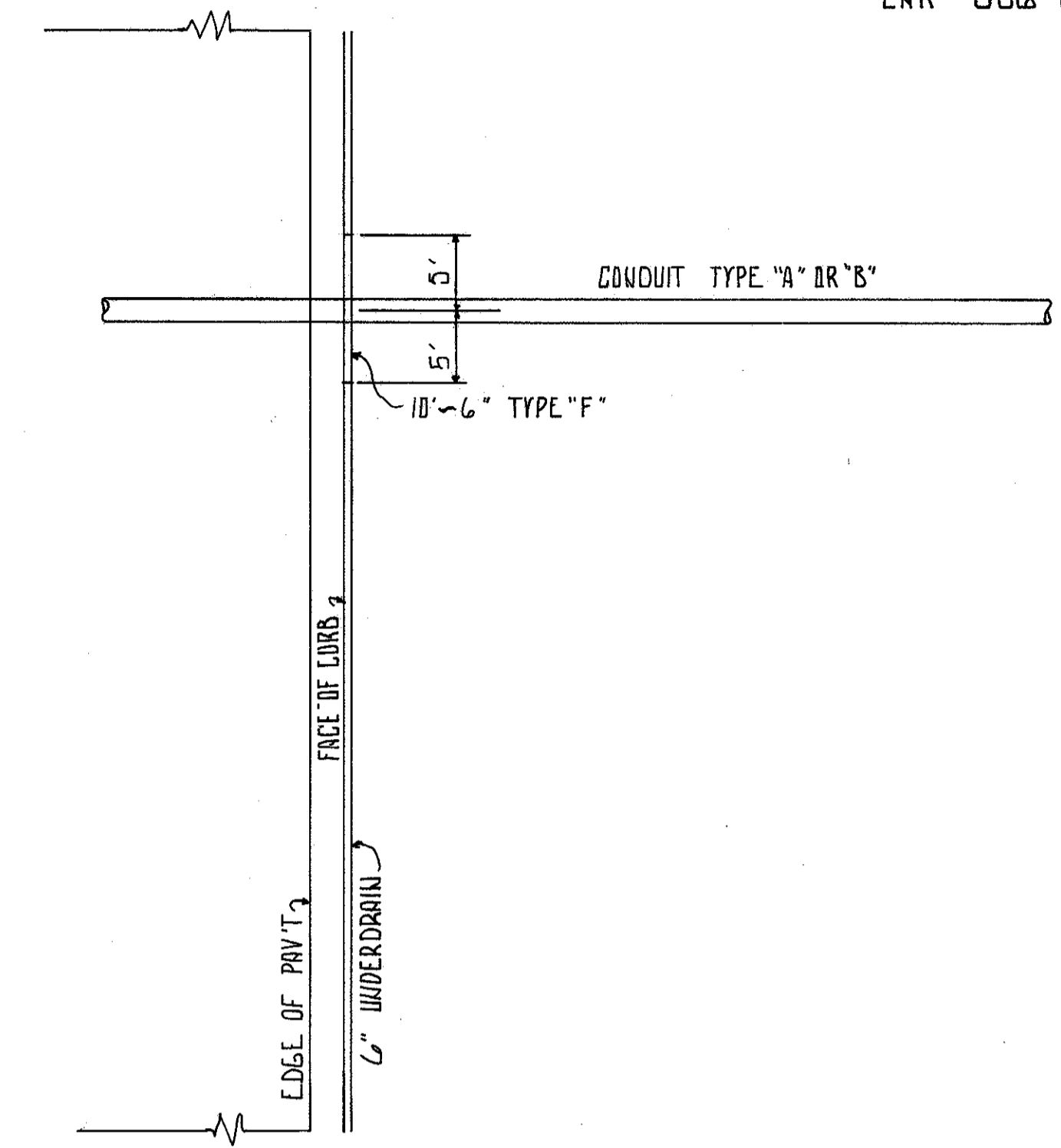
DETAIL "C"
