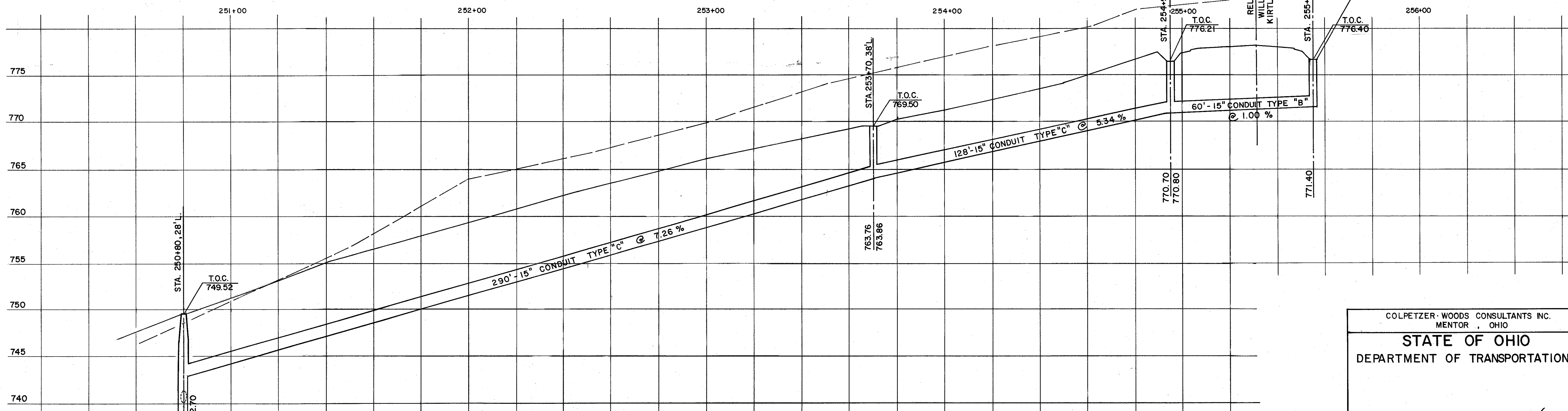
WEST SIDE STORM SEWER
