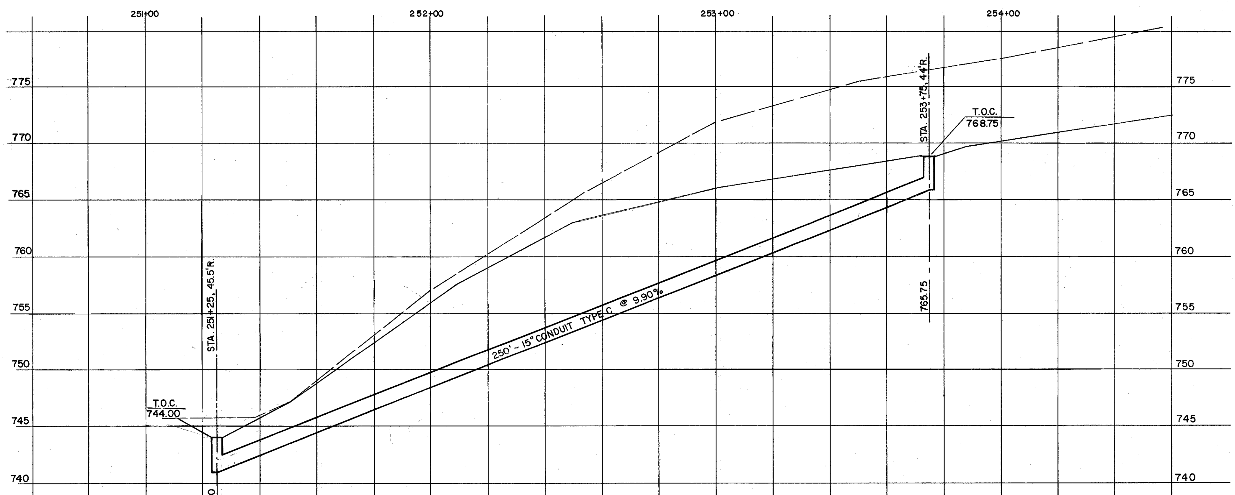
EAST SIDE STORM SEWER
