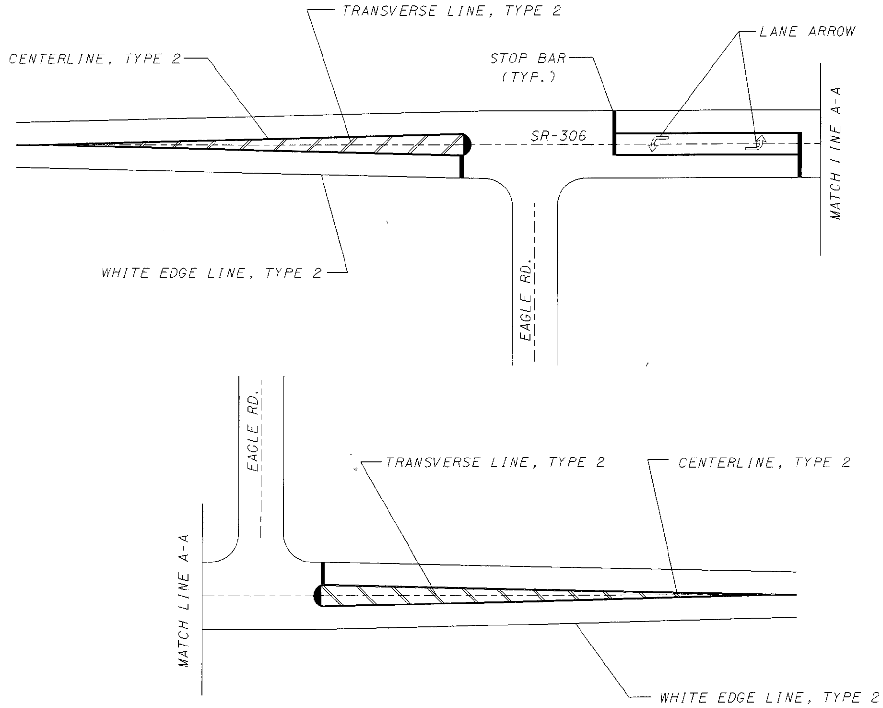
INTERSECTION DETAIL SR-306 AND EAGLE ROAD
