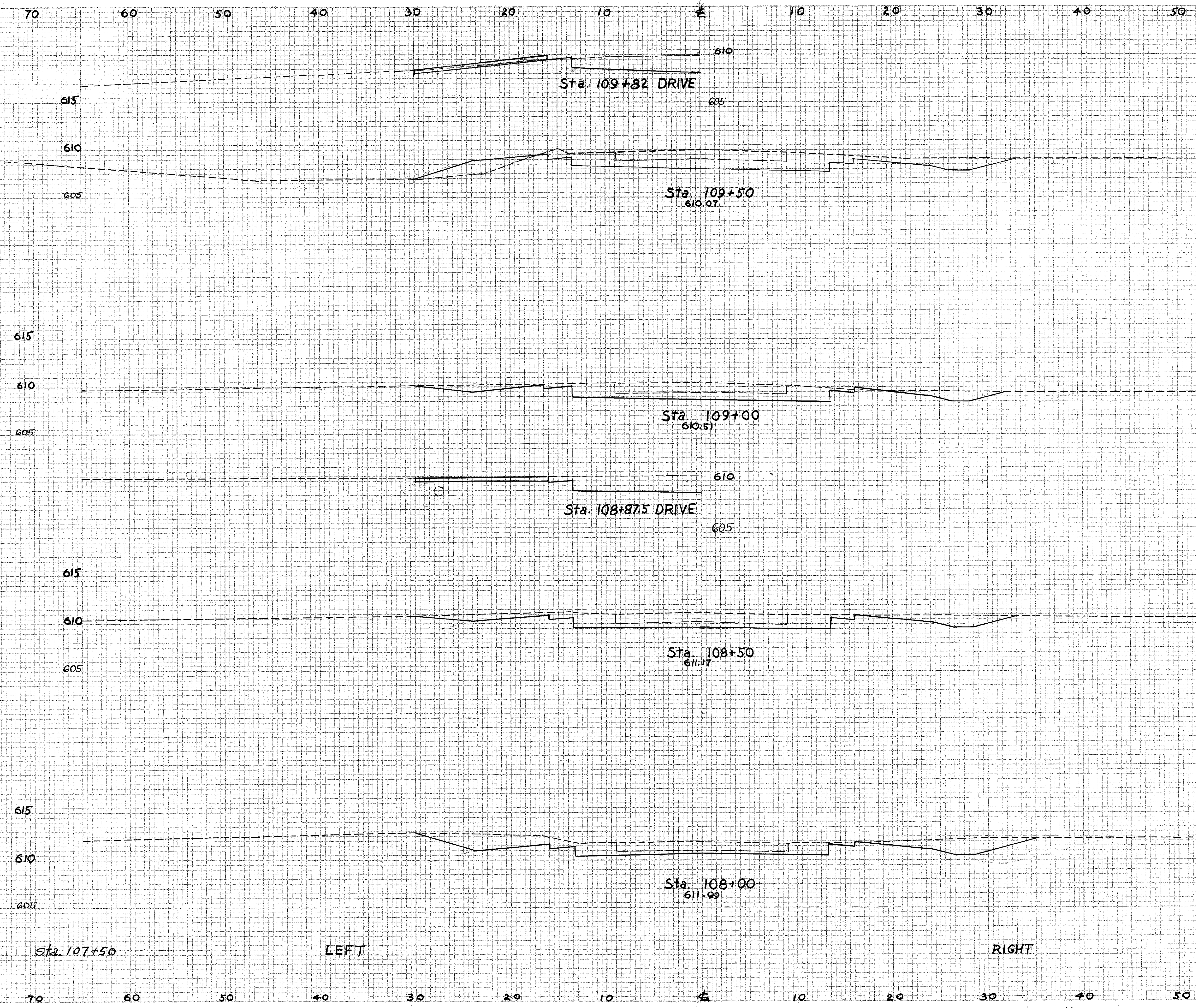
X-SECTIONS Sta. 108+00 to 109+50
