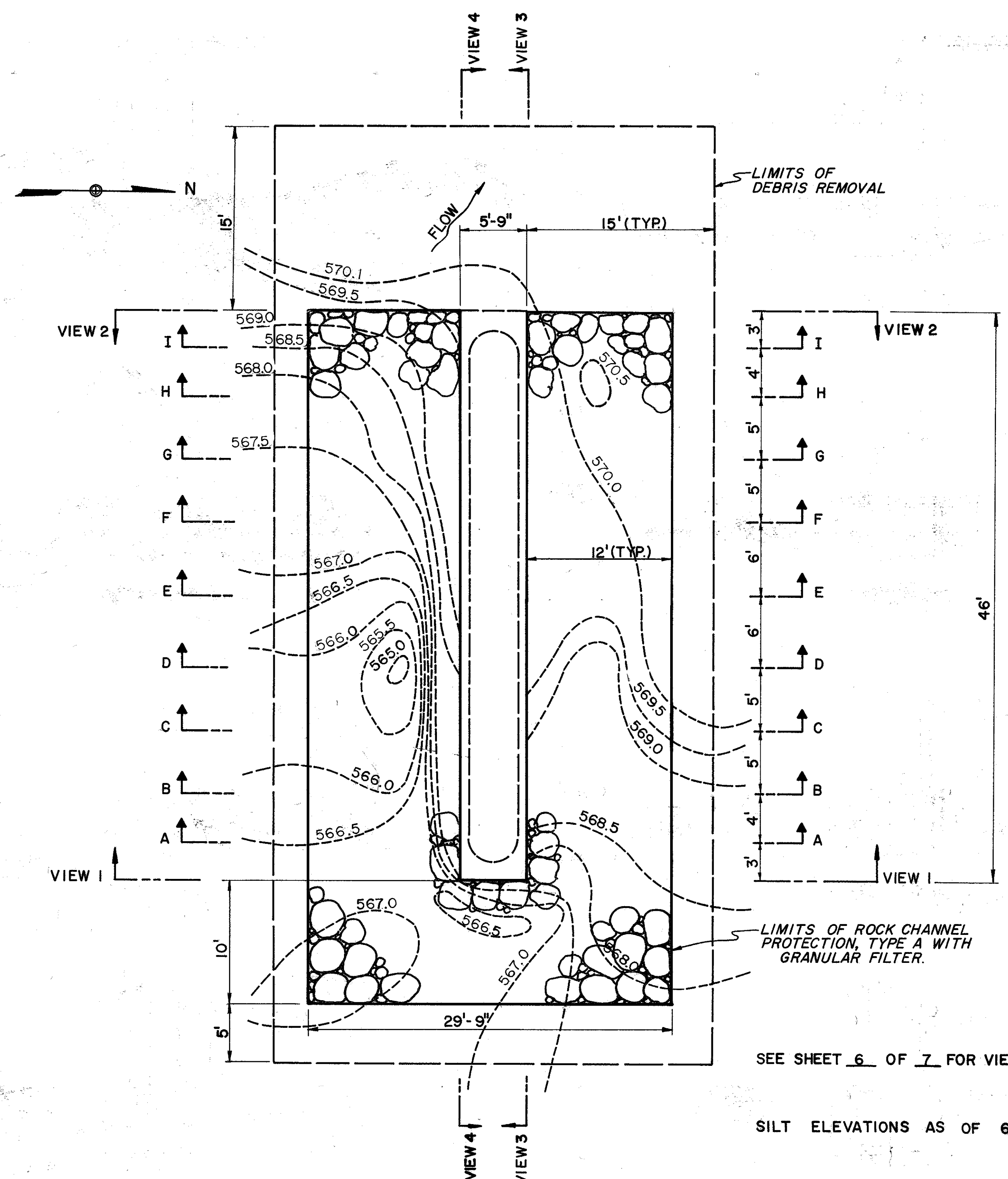
PLAN VIEW OF PIER NO. 3
