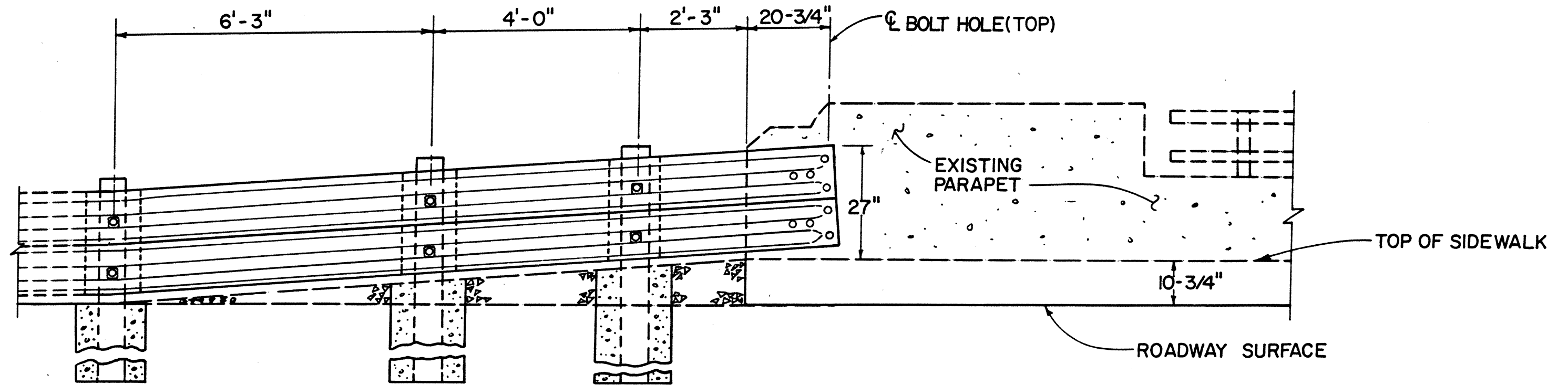
BRIDGE TERMINAL ASSEMBLY STANDARD TYPE A, DETAIL MODIFIED AS PER PLAN
