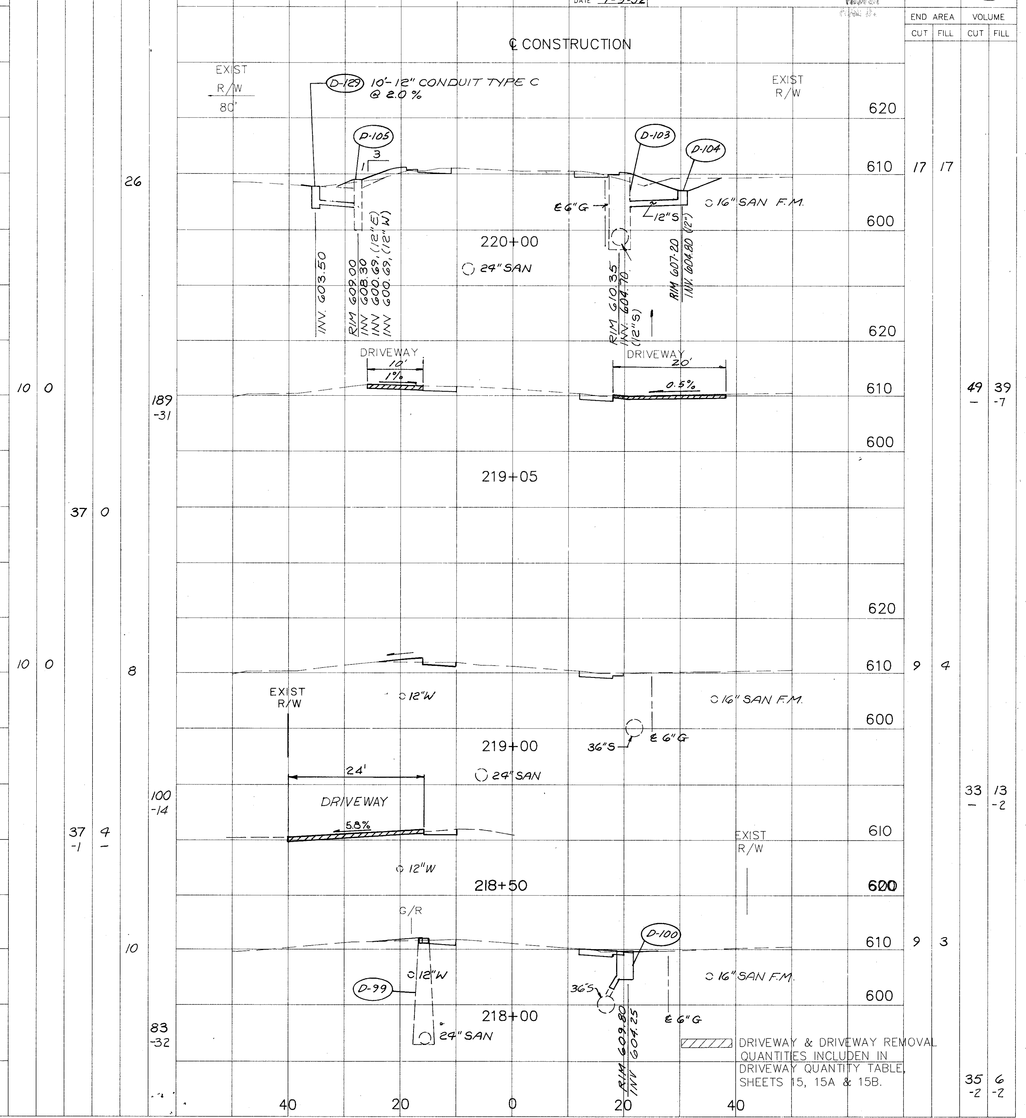
S.R. 283 X-SECTIONS STA. 215+60 TO 220+00
