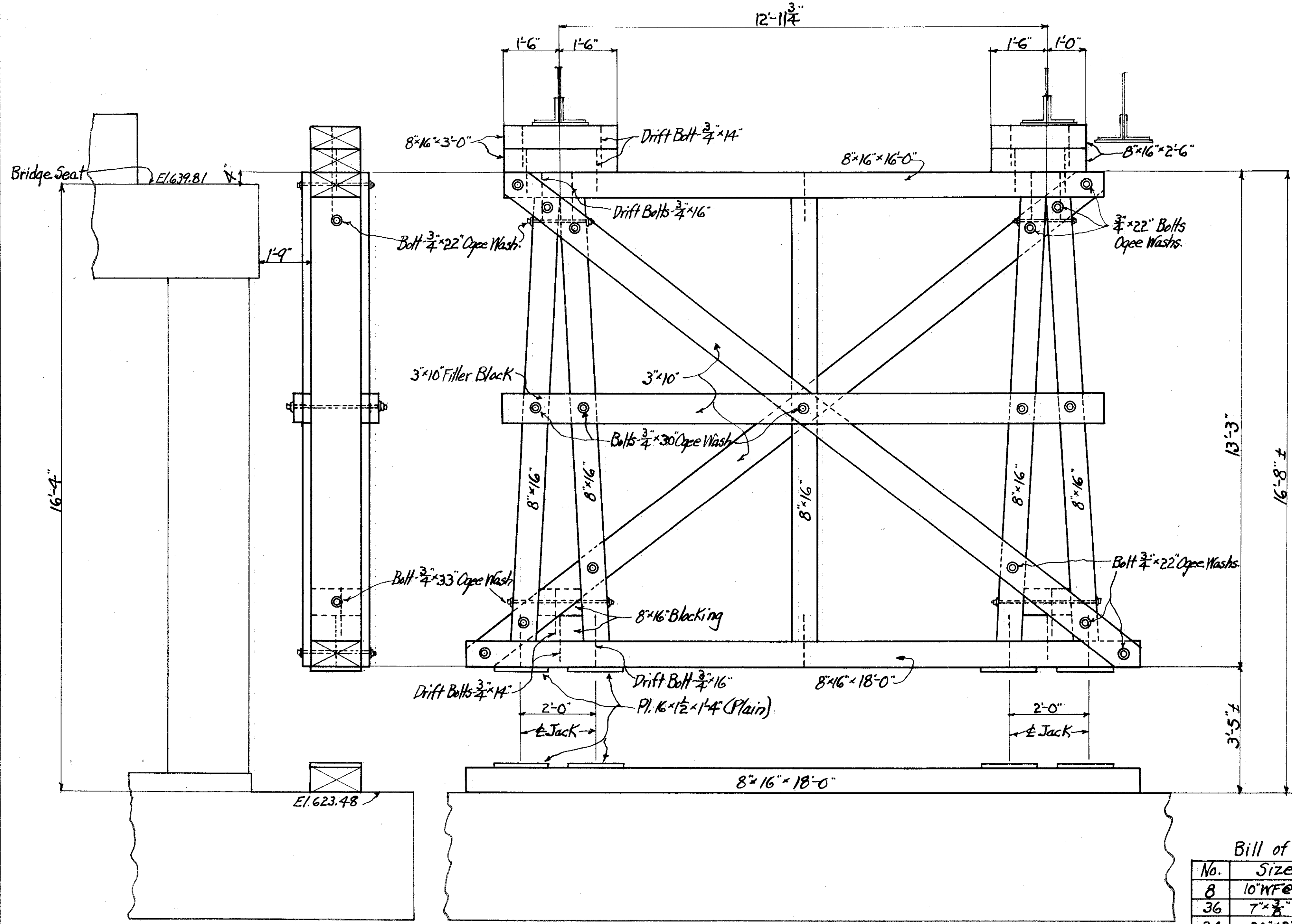
JACKING BENT DETAIL AND ASSEMBLY (Final raised position) 2-Reqd. Scale 1/2"=1'-0"
