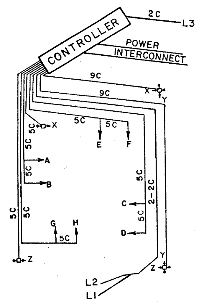
WIRING DIAGRAM
