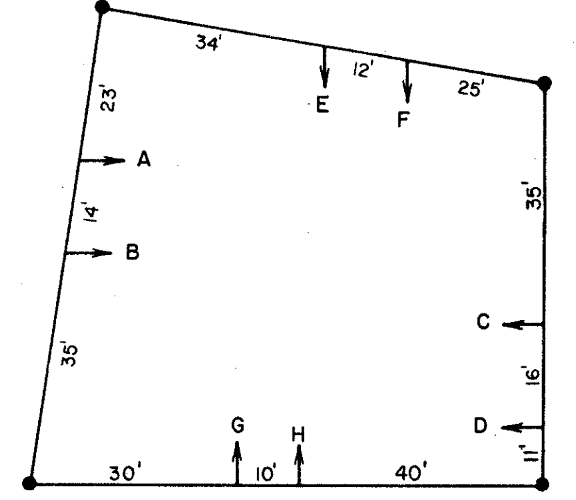
SPAN DIAGRAM
