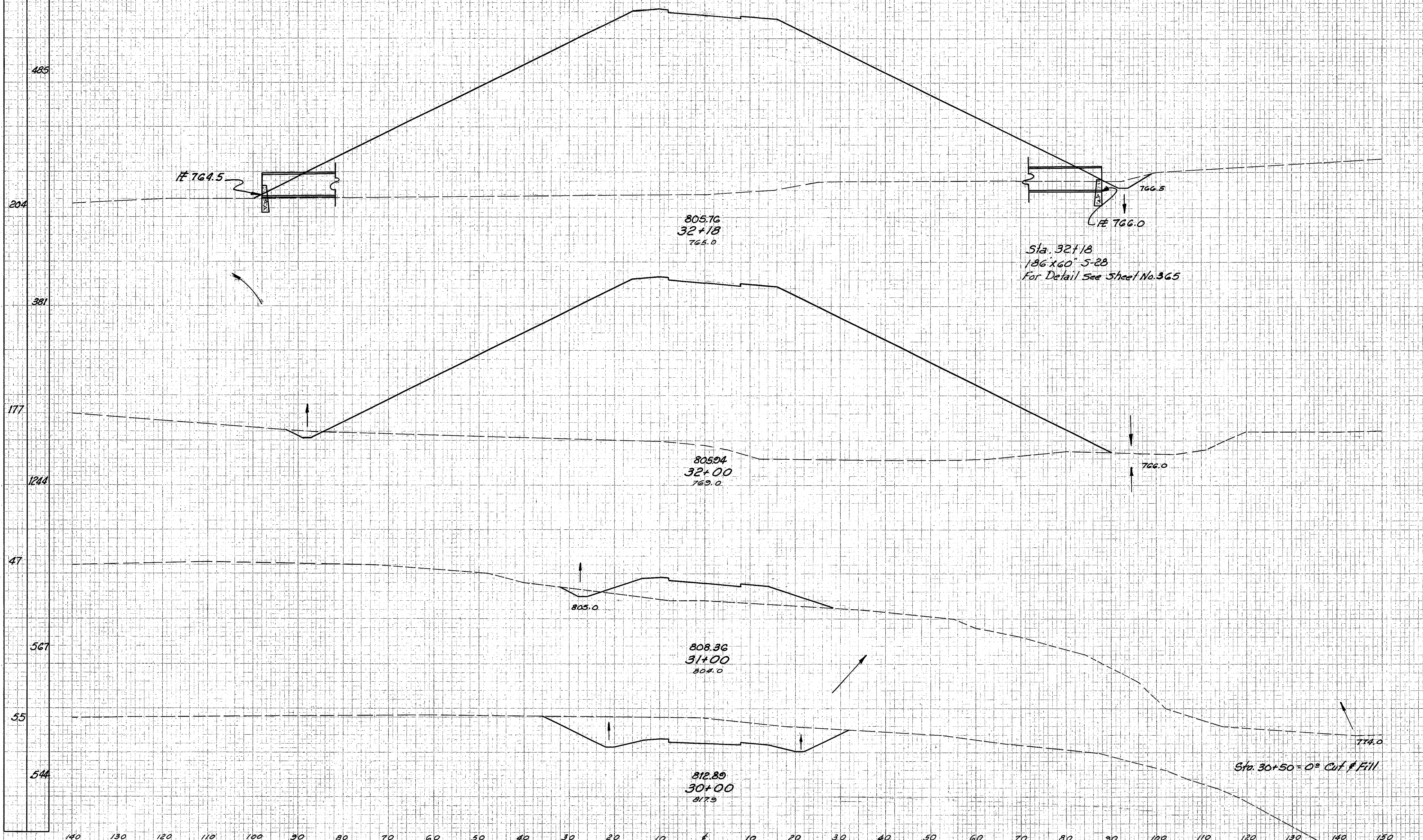
PLATE 3 - CROSS SECTION (L.A.S. & L.S. STANDARD) CHIFFEL & ASSOCIATES, NEW YORK
