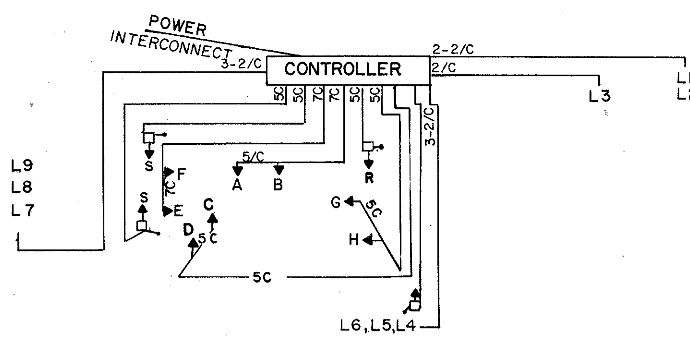
WIRING DIAGRAM
