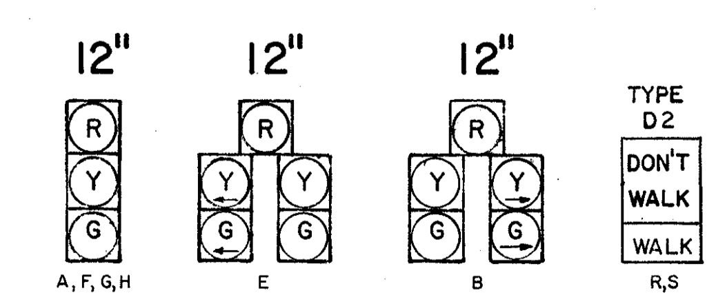
SIGNAL HEADS
