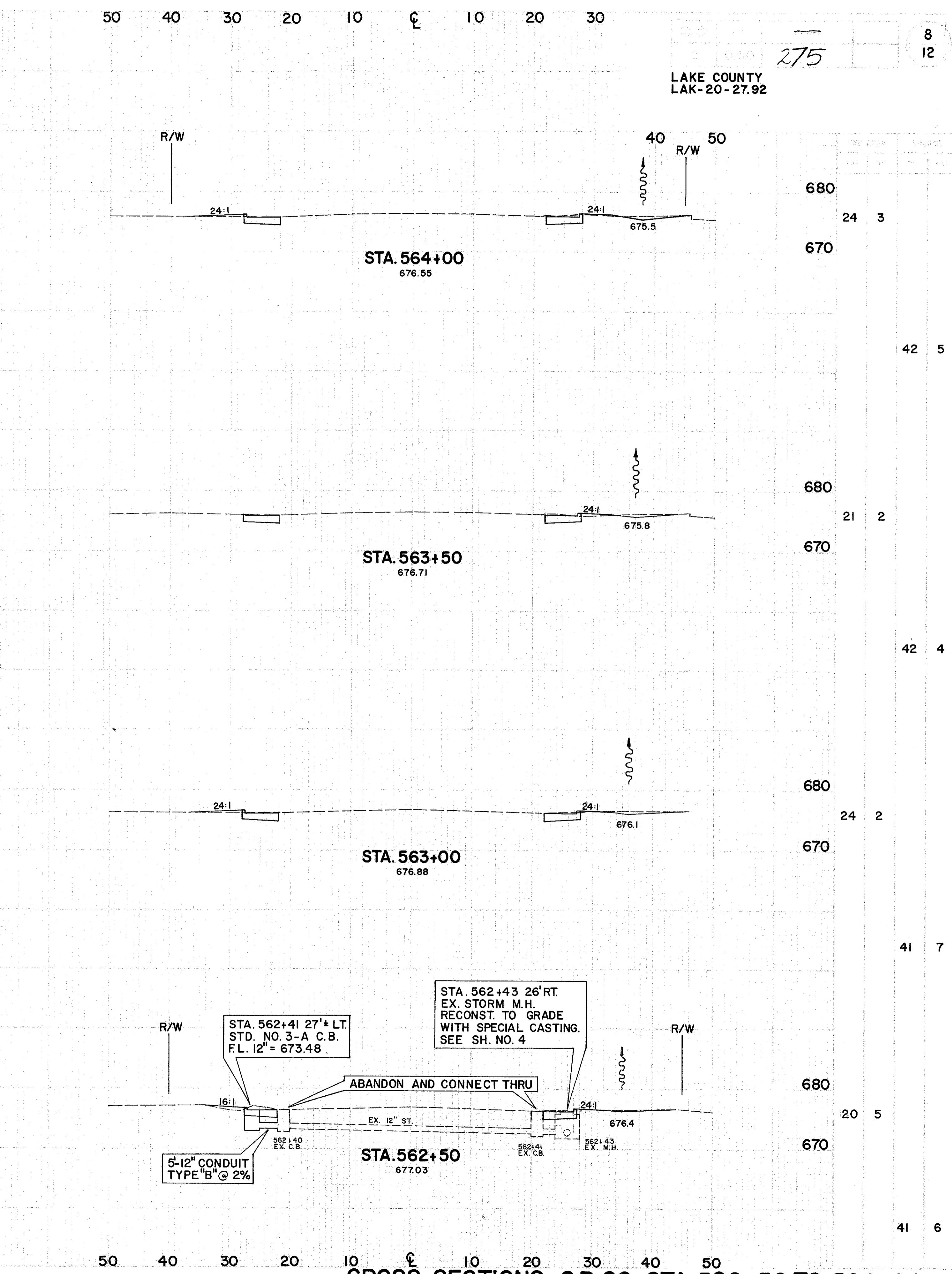
CROSS SECTIONS- S.R. 20- STA. 560+50 TO 564+00
