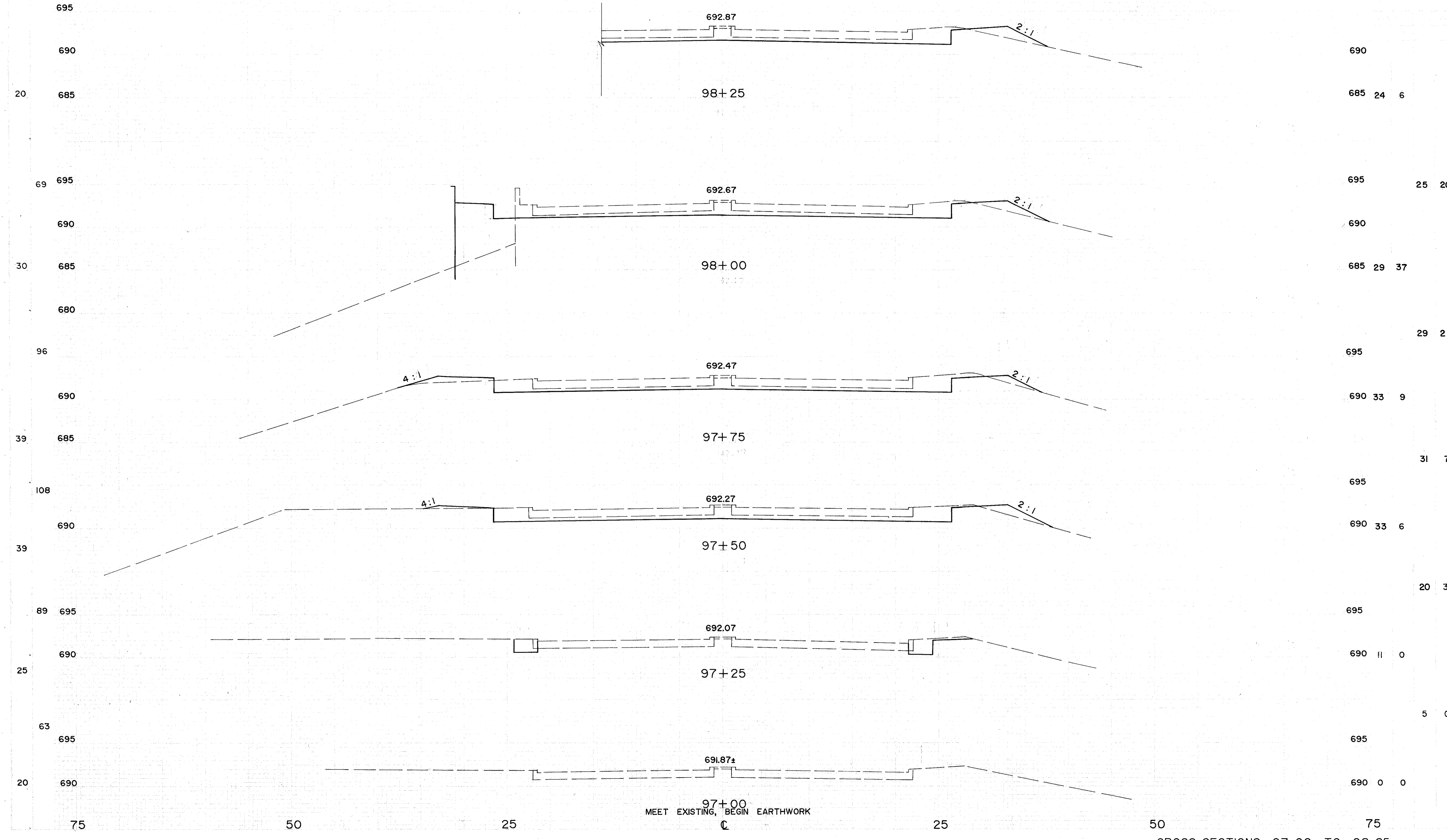
CROSS SECTIONS 97+00 TO 98+25
