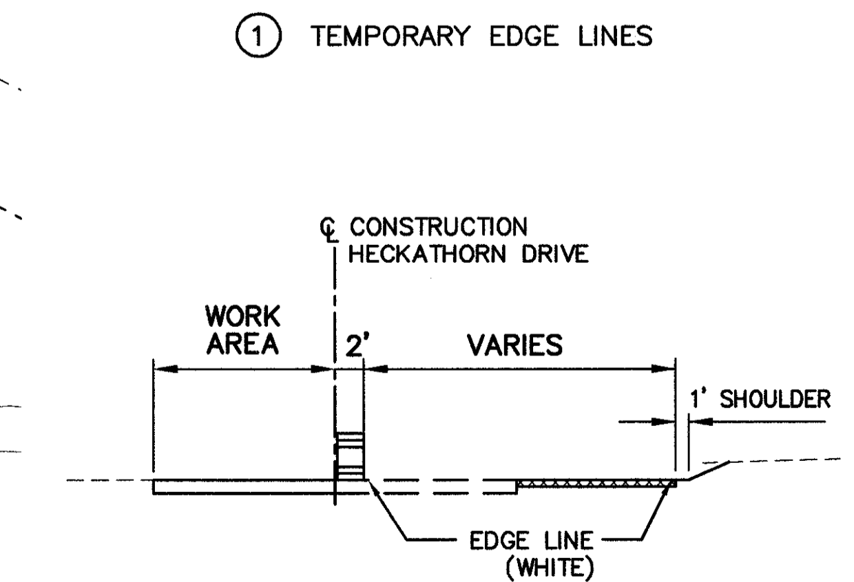
PART B TYPICAL SECTION
