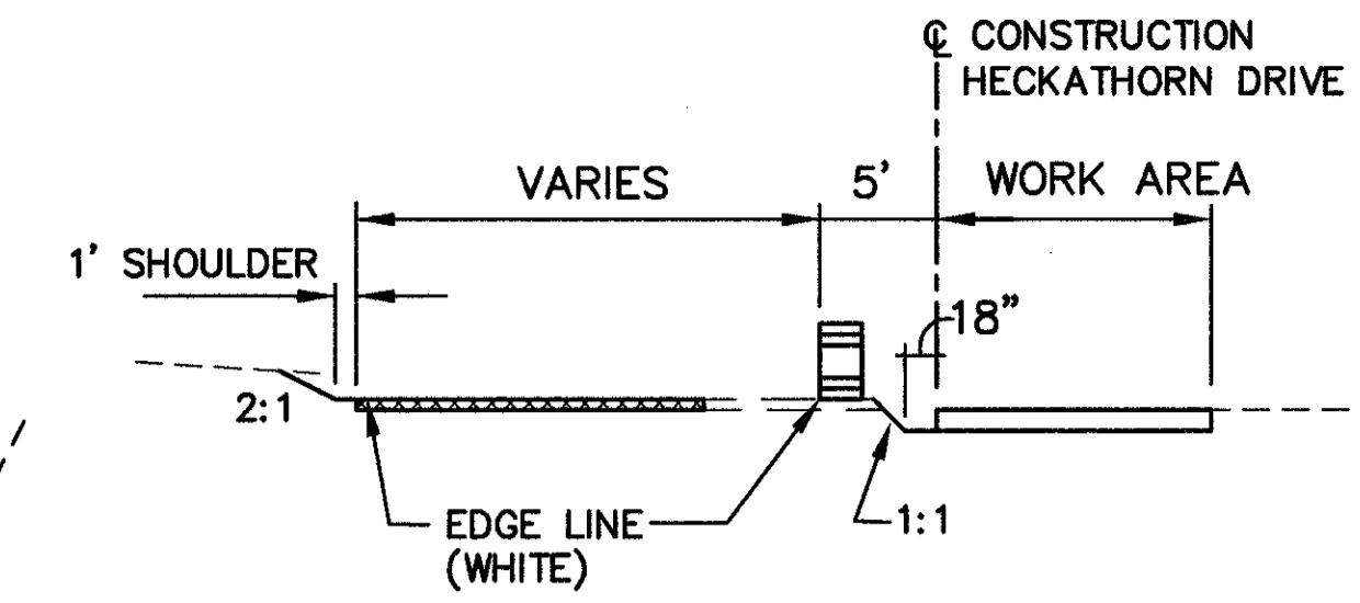
PART A TYPICAL SECTION
