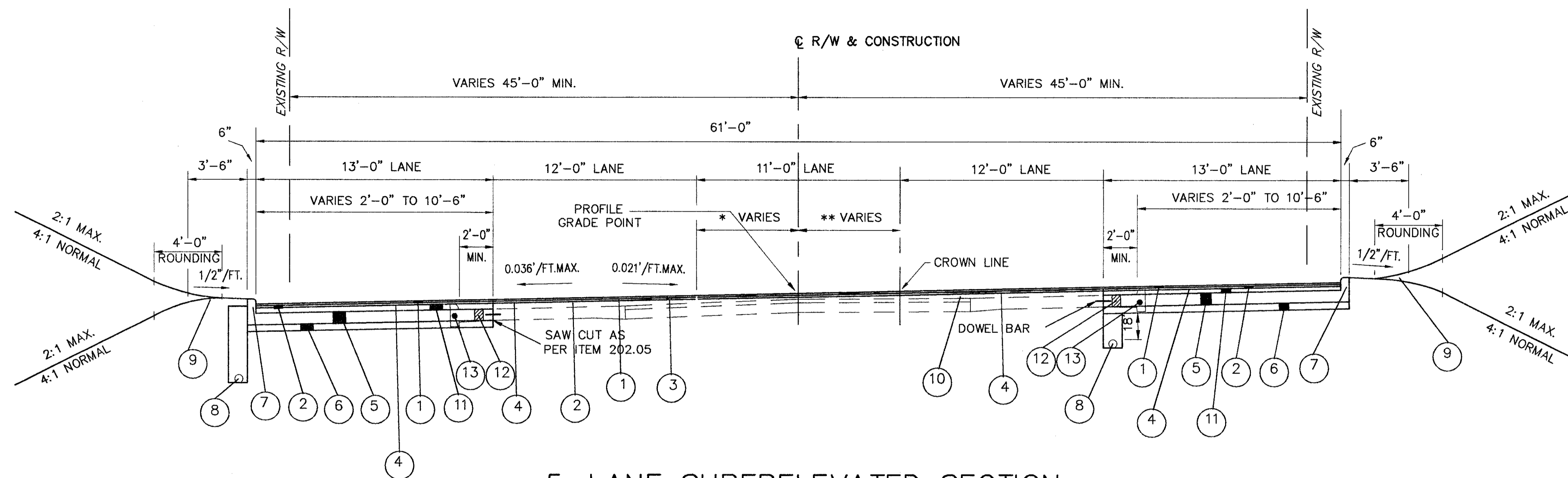
5-LANE SUPERELEVATED SECTION (SYMMETRICAL WIDENING)
