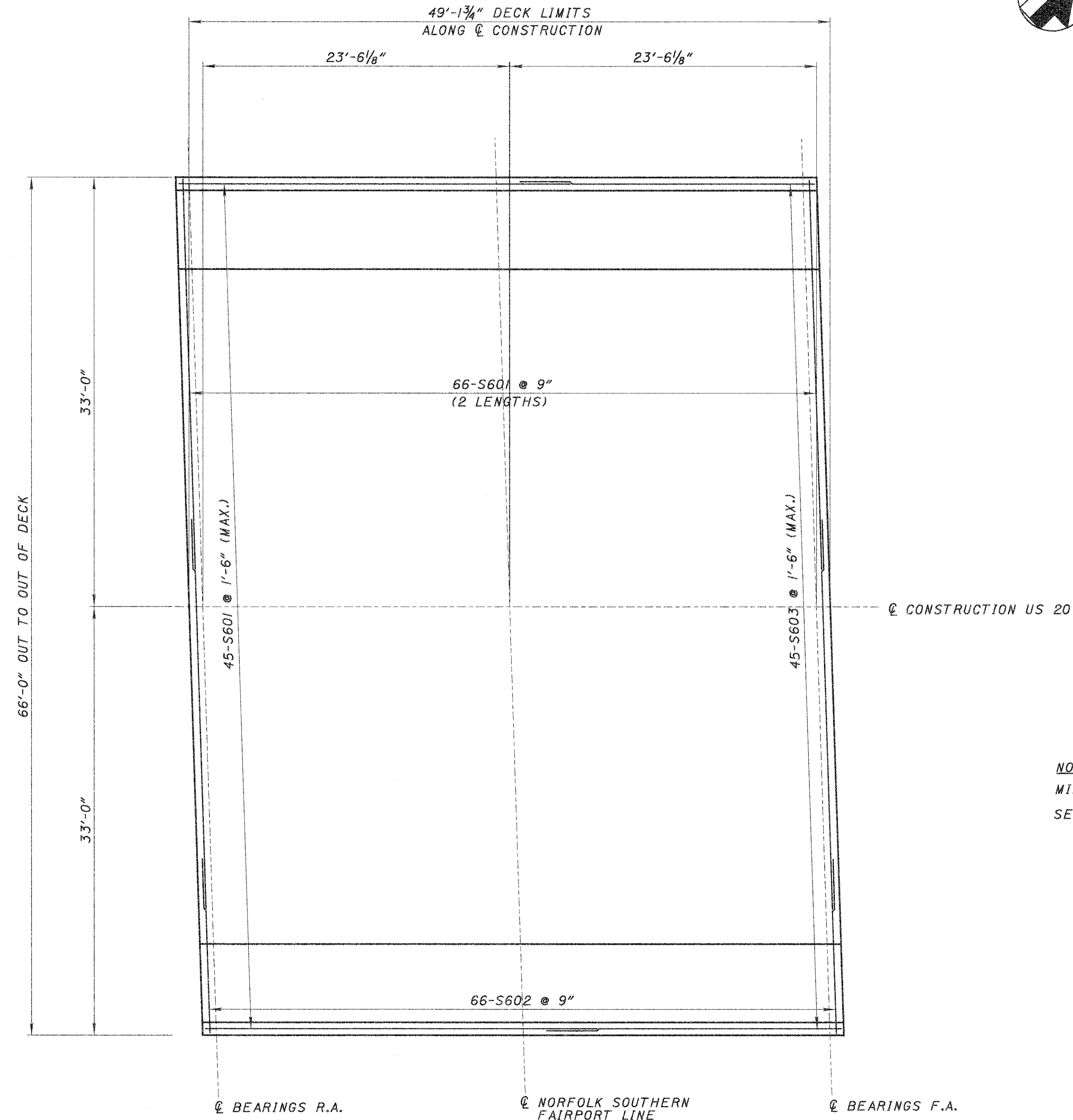
DECK SLAB PLAN
