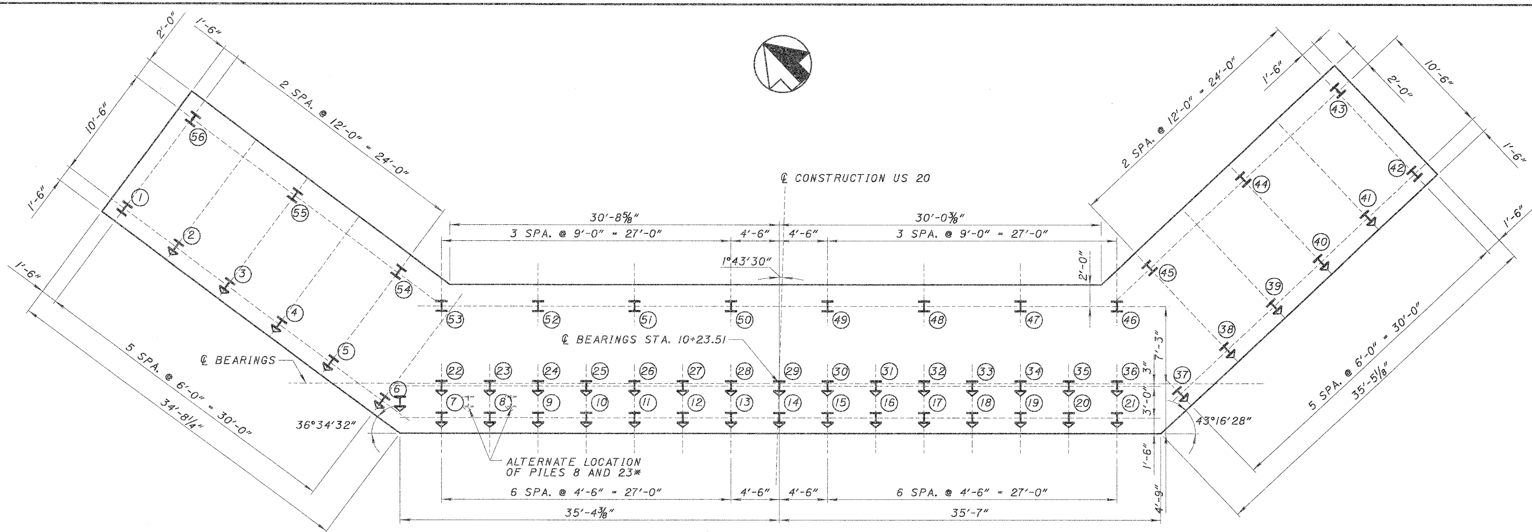
FORWARD ABUTMENT FOUNDATION PLAN
