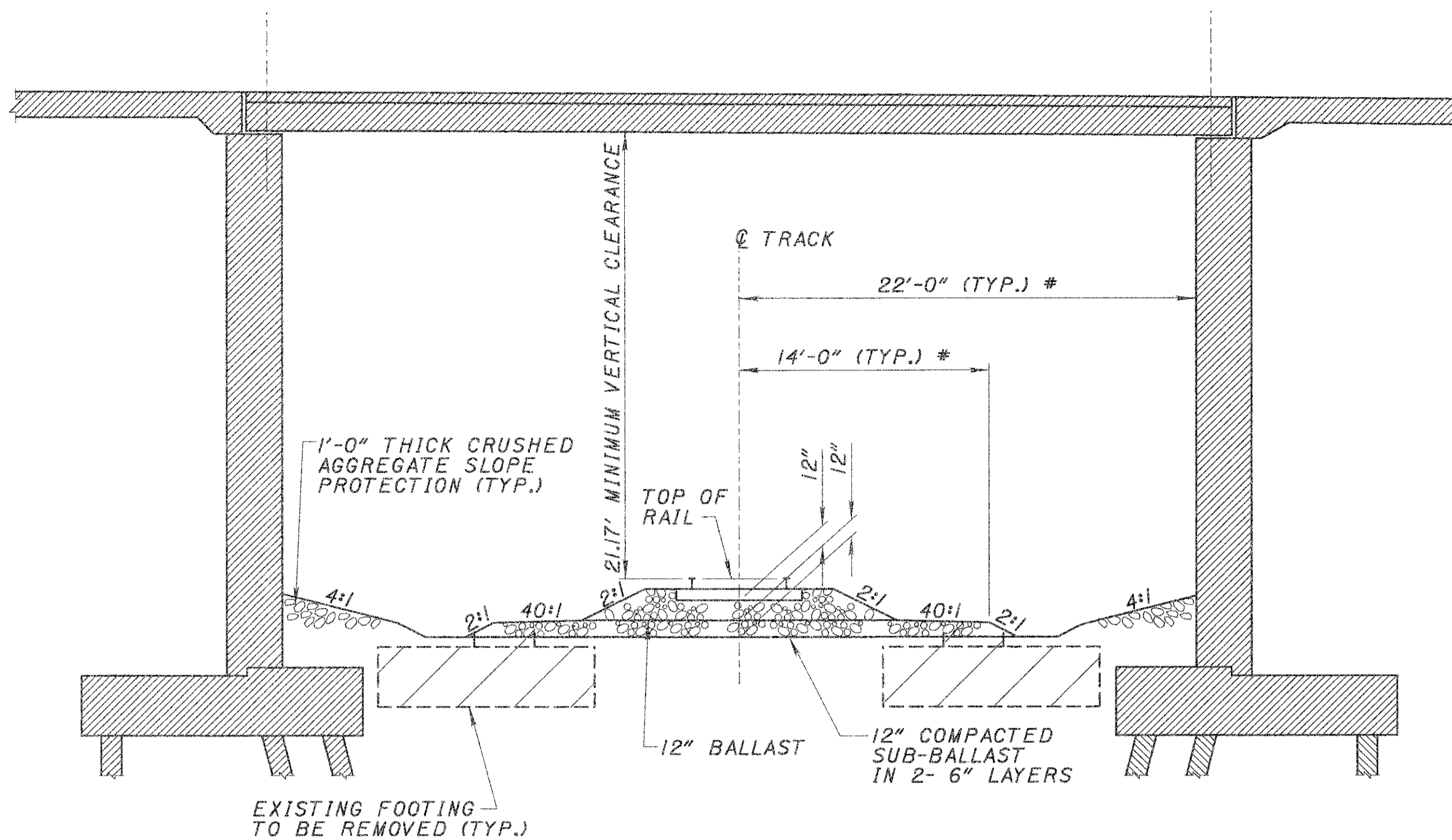
PROPOSED TRACK TYPICAL SECTION AT BRIDGE & DITCH DETAIL
