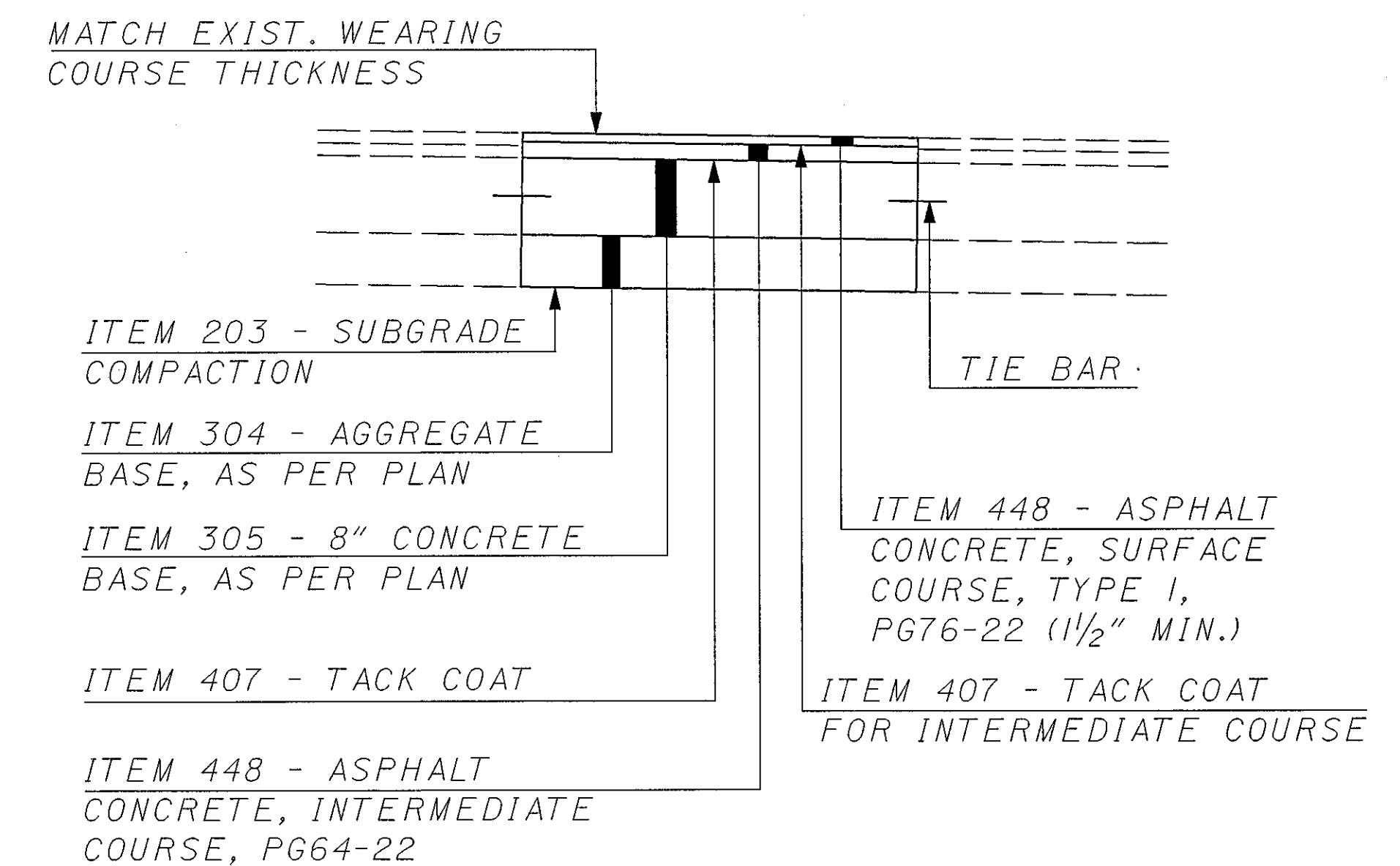
TRENCH REPAIR DETAIL
